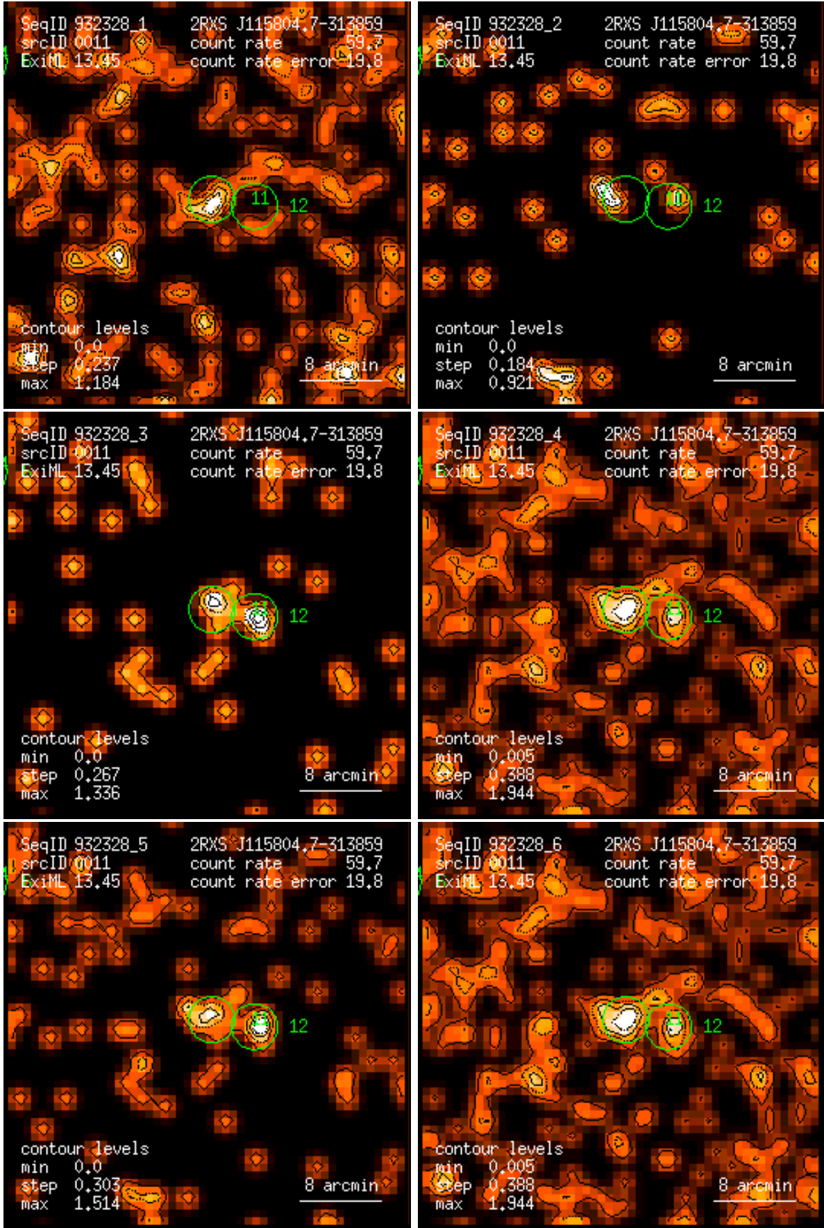
Figure 11: RASS 932328: detection 0011: band rate images, Gaussian filter: (1) PSPC channels 11 – 41, (2) 52 – 90, (3) 91 – 201, (4) 11 – 235, (5) 52 – 201, (6) 11 – 201. Broad band rates in counts/ks. Band rate contour levels in counts/ks/arcmin 2 .
