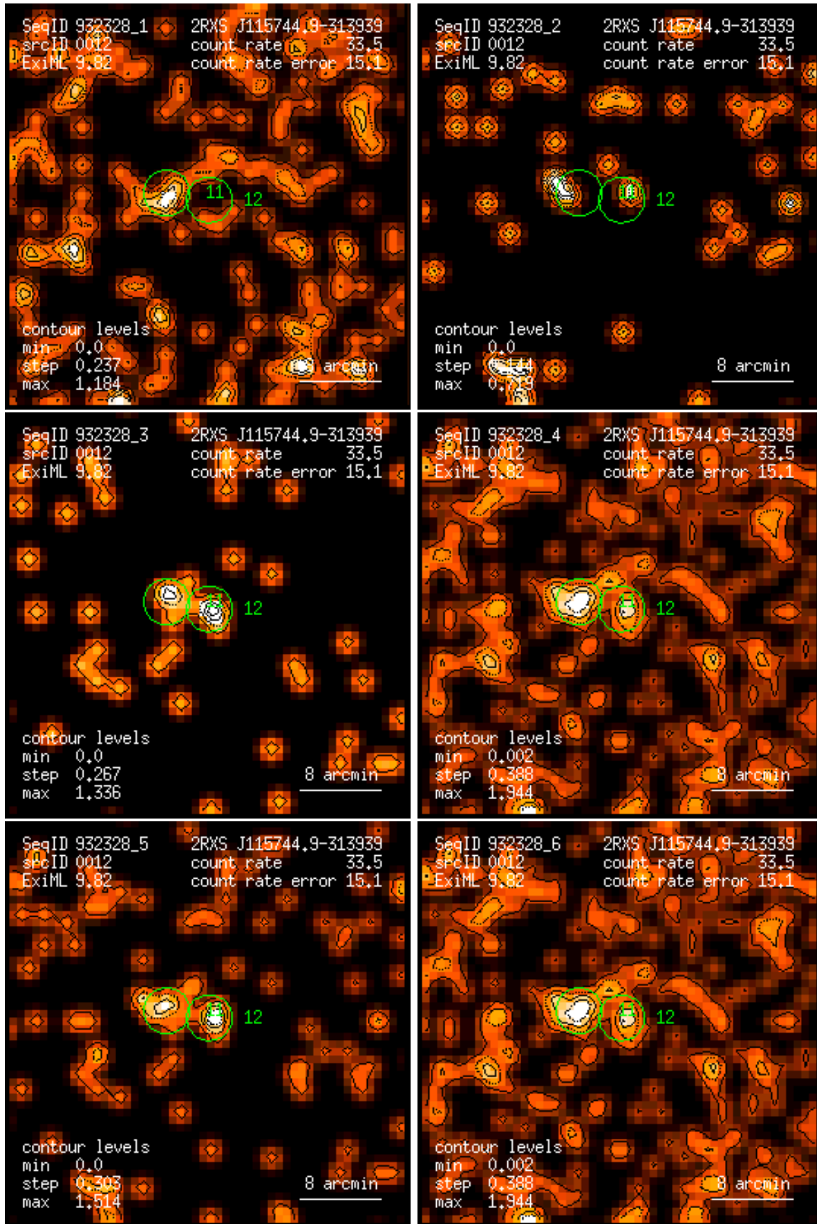
Figure 12: RASS 932328: detection 0012: band rate images, Gaussian filter: (1) PSPC channels 11 – 41, (2) 52 – 90, (3) 91 – 201, (4) 11 – 235, (5) 52 – 201, (6) 11 – 201. Broad band rates in counts/ks. Band rate contour levels in counts/ks/arcmin 2 .
