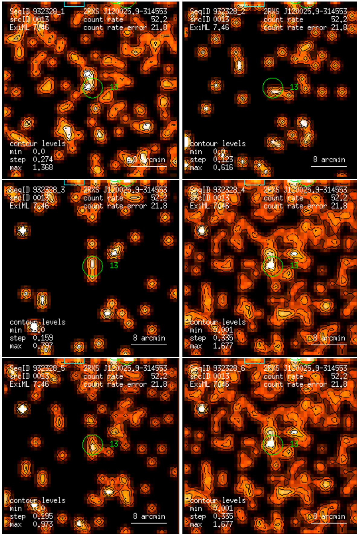
Figure 13: RASS 932328: detection 0013: band rate images, Gaussian filter: (1) PSPC channels 11 – 41, (2) 52 – 90, (3) 91 – 201, (4) 11 – 235, (5) 52 – 201, (6) 11 – 201. Broad band rates in counts/ks. Band rate contour levels in counts/ks/arcmin 2 .
