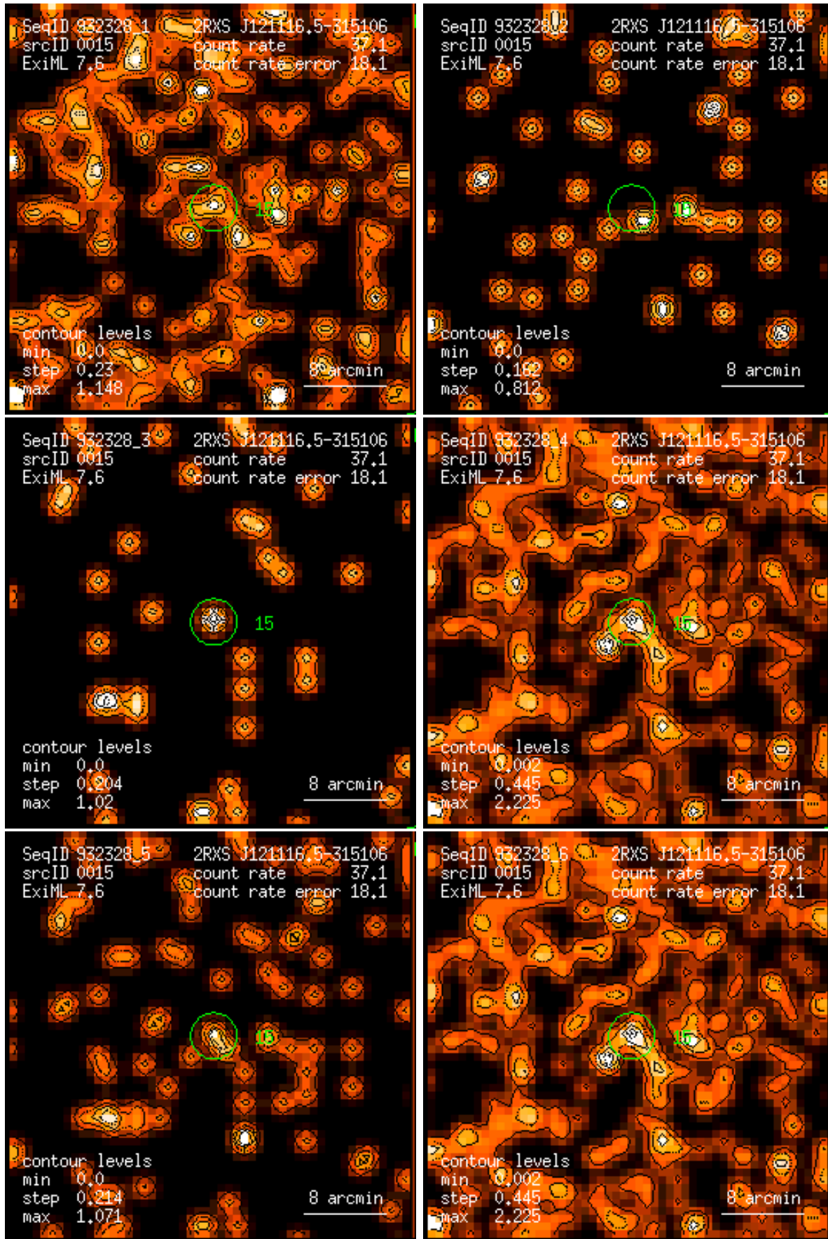
Figure 15: RASS 932328: detection 0015: band rate images, Gaussian filter: (1) PSPC channels 11 – 41, (2) 52 – 90, (3) 91 – 201, (4) 11 – 235, (5) 52 – 201, (6) 11 – 201. Broad band rates in counts/ks. Band rate contour levels in counts/ks/arcmin 2 .
