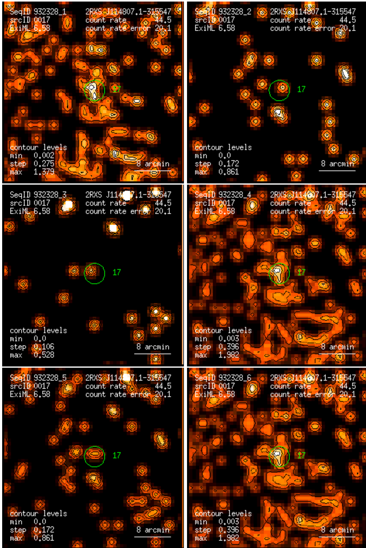
Figure 17: RASS 932328: detection 0017: band rate images, Gaussian filter: (1) PSPC channels 11 – 41, (2) 52 – 90, (3) 91 – 201, (4) 11 – 235, (5) 52 – 201, (6) 11 – 201. Broad band rates in counts/ks. Band rate contour levels in counts/ks/arcmin 2 .
