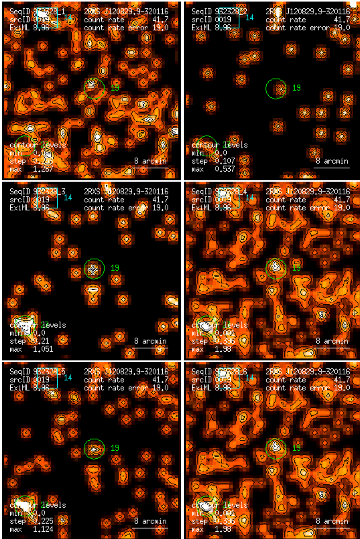
Figure 19: RASS 932328: detection 0019: band rate images, Gaussian filter: (1) PSPC channels 11 – 41, (2) 52 – 90, (3) 91 – 201, (4) 11 – 235, (5) 52 – 201, (6) 11 – 201. Broad band rates in counts/ks. Band rate contour levels in counts/ks/arcmin 2 .
