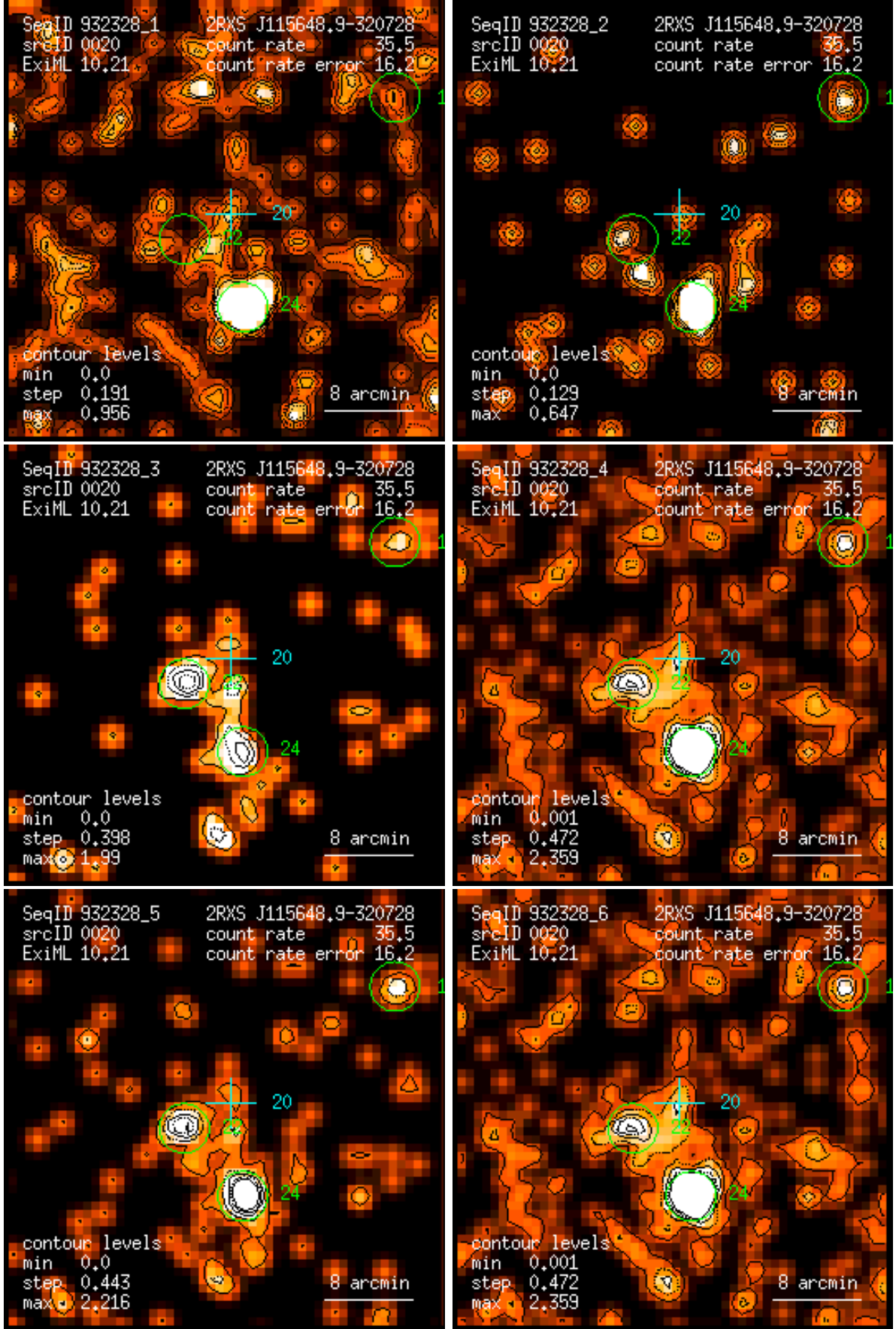
Figure 20: RASS 932328: detection 0020: band rate images, Gaussian filter: (1) PSPC channels 11 – 41, (2) 52 – 90, (3) 91 – 201, (4) 11 – 235, (5) 52 – 201, (6) 11 – 201. Broad band rates in counts/ks. Band rate contour levels in counts/ks/arcmin 2 .
