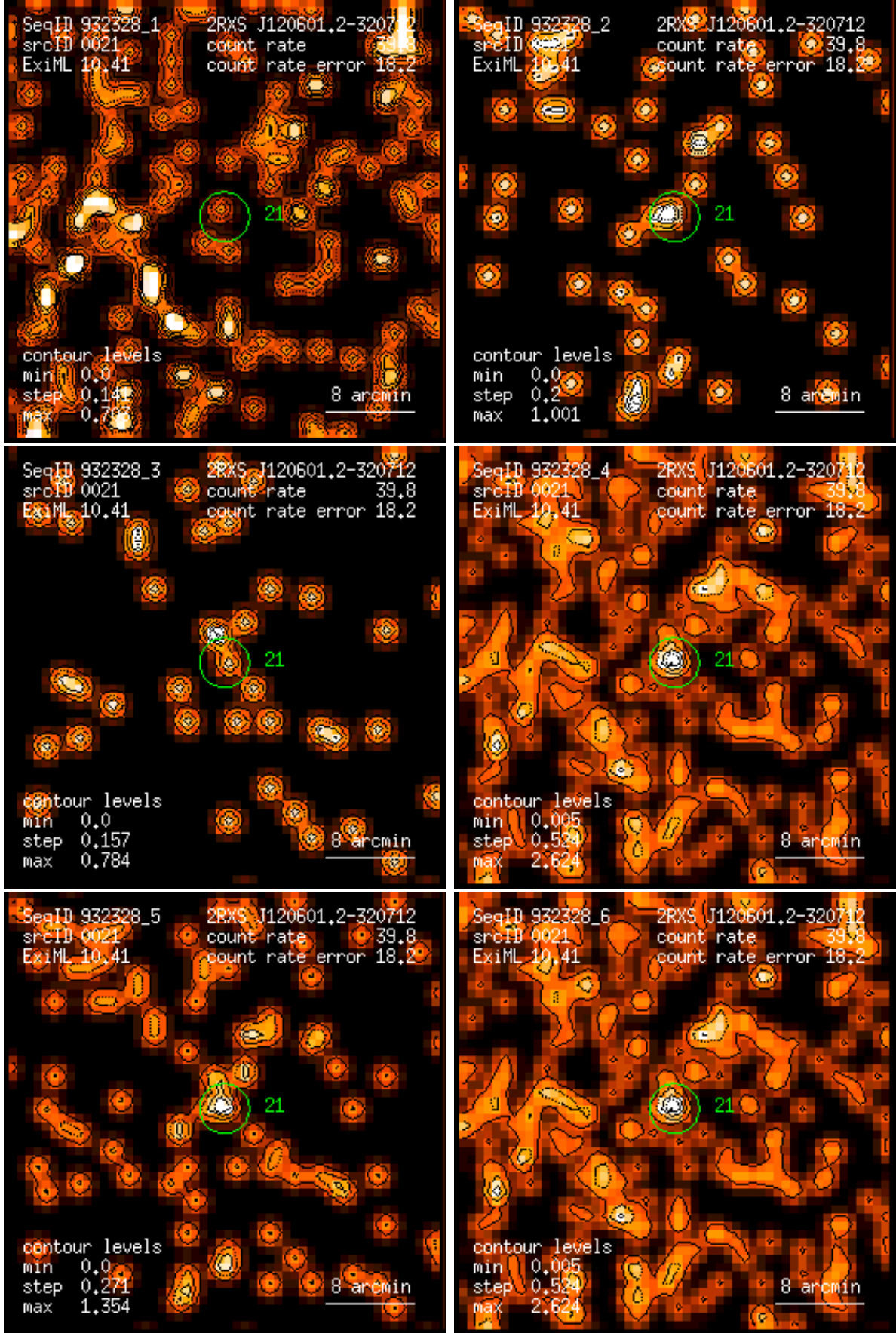
Figure 21: RASS 932328: detection 0021: band rate images, Gaussian filter: (1) PSPC channels 11 – 41, (2) 52 – 90, (3) 91 – 201, (4) 11 – 235, (5) 52 – 201, (6) 11 – 201. Broad band rates in counts/ks. Band rate contour levels in counts/ks/arcmin 2 .
