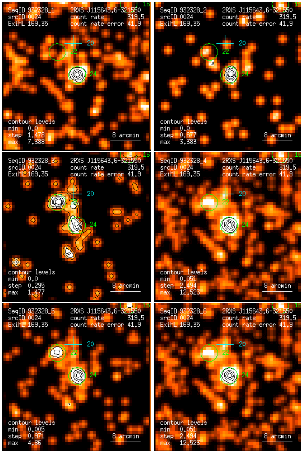
Figure 24: RASS 932328: detection 0024: band rate images, Gaussian filter: (1) PSPC channels 11 – 41, (2) 52 – 90, (3) 91 – 201, (4) 11 – 235, (5) 52 – 201, (6) 11 – 201. Broad band rates in counts/ks. Band rate contour levels in counts/ks/arcmin 2 .
