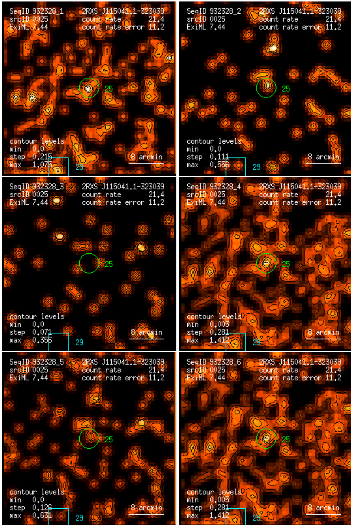
Figure 25: RASS 932328: detection 0025: band rate images, Gaussian filter: (1) PSPC channels 11 – 41, (2) 52 – 90, (3) 91 – 201, (4) 11 – 235, (5) 52 – 201, (6) 11 – 201. Broad band rates in counts/ks. Band rate contour levels in counts/ks/arcmin 2 .
