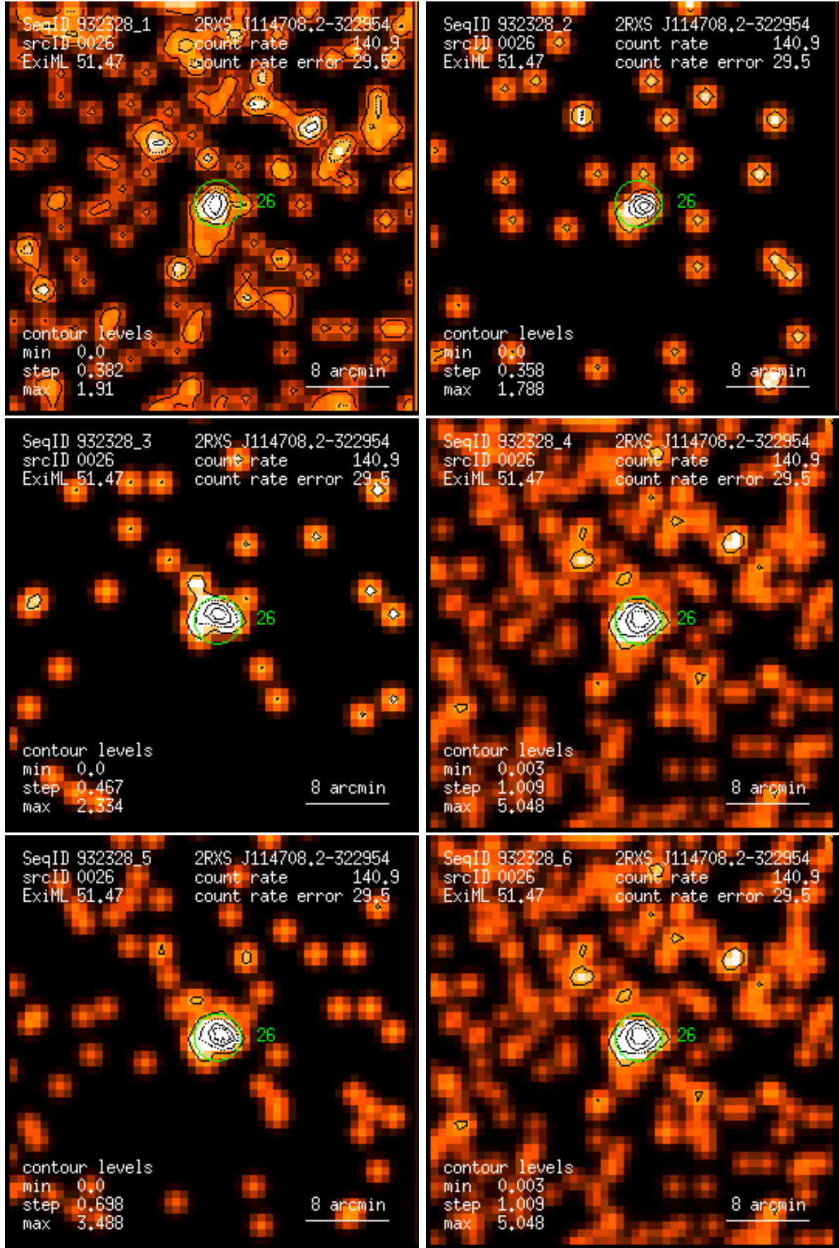
Figure 26: RASS 932328: detection 0026: band rate images, Gaussian filter: (1) PSPC channels 11 – 41, (2) 52 – 90, (3) 91 – 201, (4) 11 – 235, (5) 52 – 201, (6) 11 – 201. Broad band rates in counts/ks. Band rate contour levels in counts/ks/arcmin 2 .
