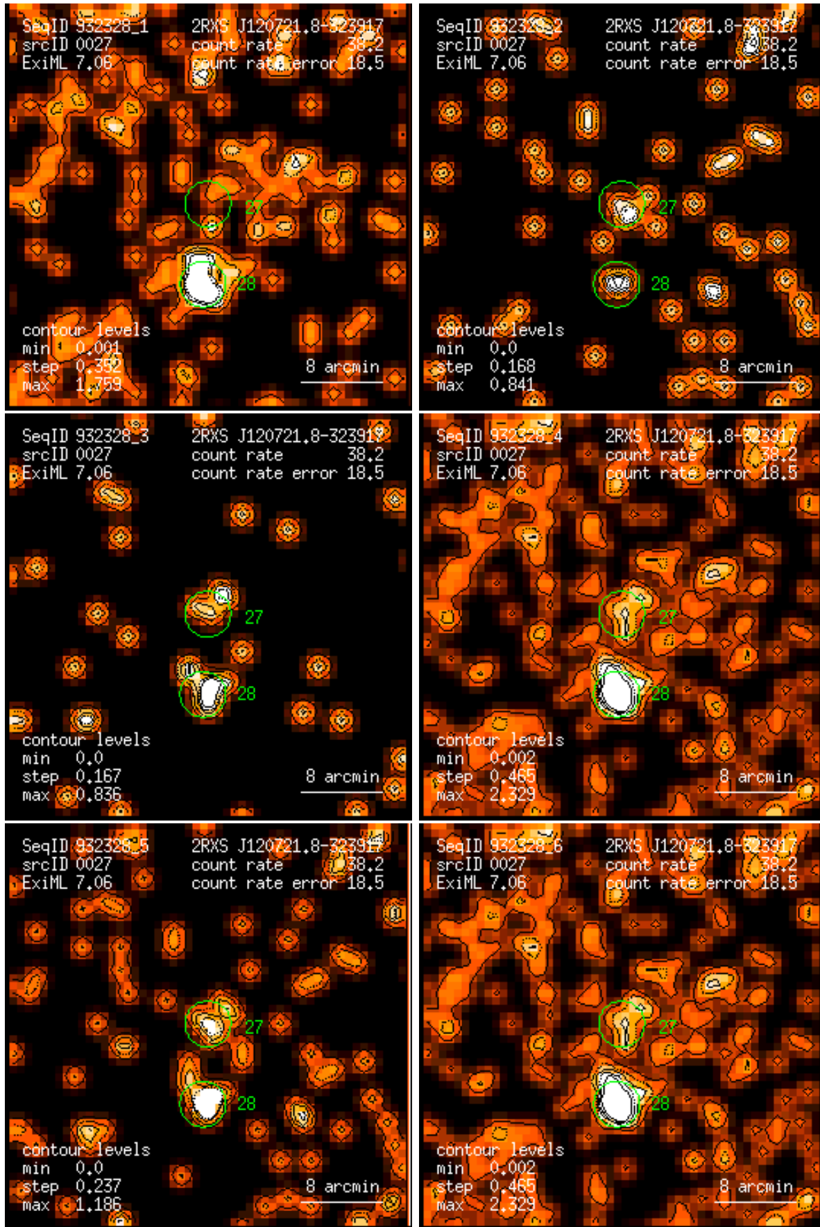
Figure 27: RASS 932328: detection 0027: band rate images, Gaussian filter: (1) PSPC channels 11 – 41, (2) 52 – 90, (3) 91 – 201, (4) 11 – 235, (5) 52 – 201, (6) 11 – 201. Broad band rates in counts/ks. Band rate contour levels in counts/ks/arcmin 2 .
