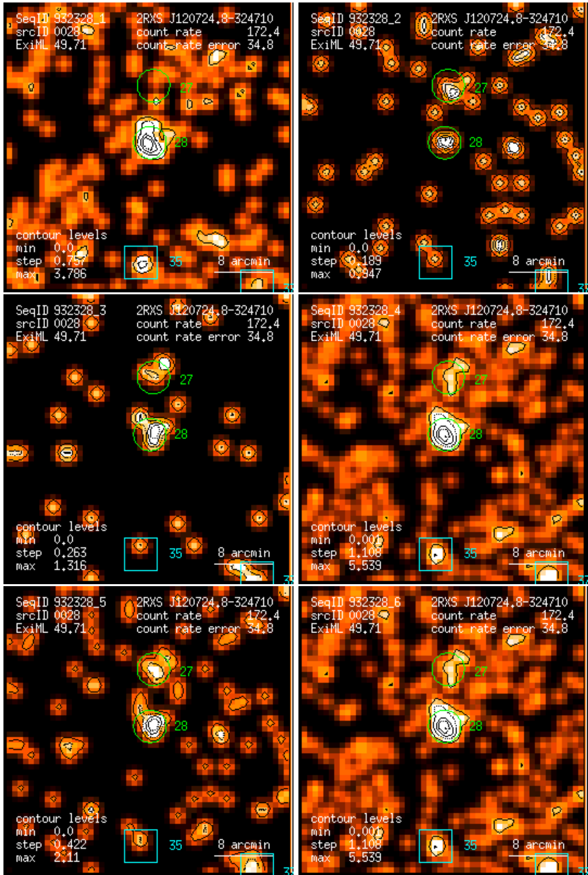
Figure 28: RASS 932328: detection 0028: band rate images, Gaussian filter: (1) PSPC channels 11 – 41, (2) 52 – 90, (3) 91 – 201, (4) 11 – 235, (5) 52 – 201, (6) 11 – 201. Broad band rates in counts/ks. Band rate contour levels in counts/ks/arcmin 2 .
