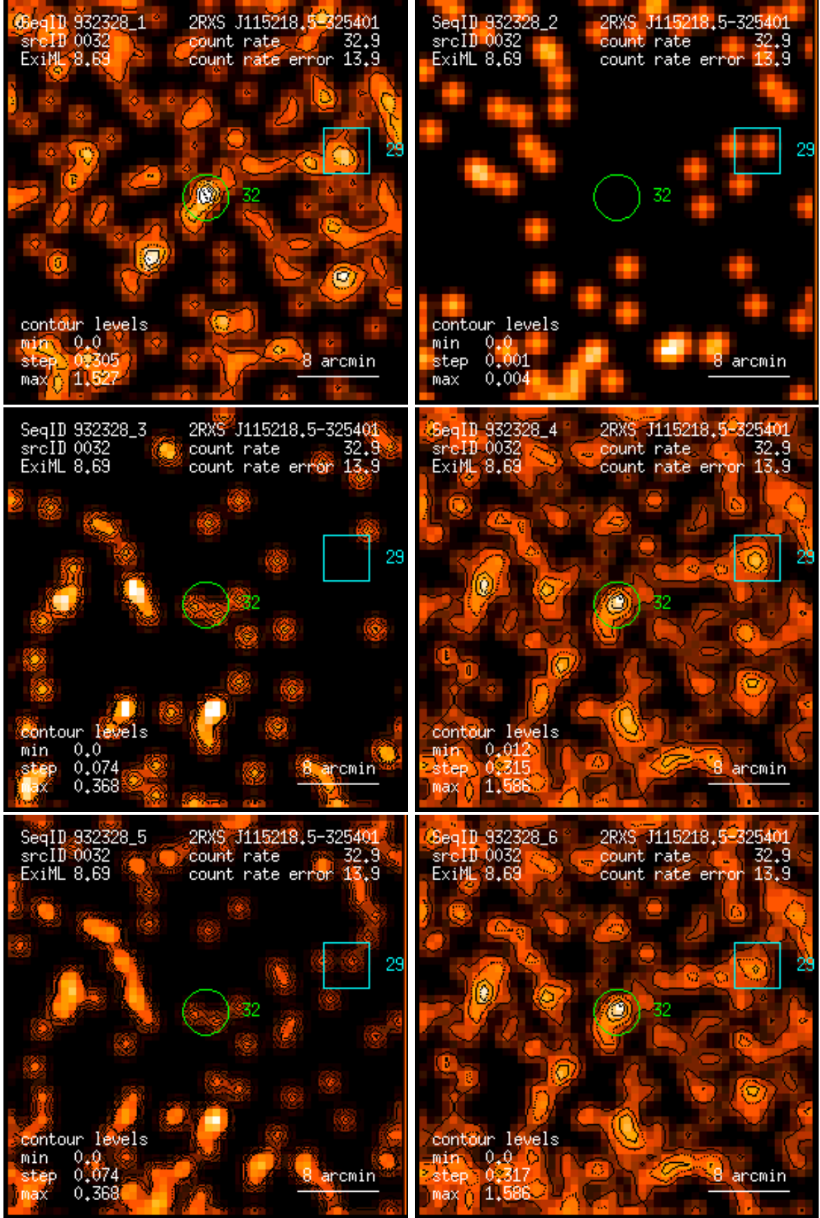
Figure 32: RASS 932328: detection 0032: band rate images, Gaussian filter: (1) PSPC channels 11 – 41, (2) 52 – 90, (3) 91 – 201, (4) 11 – 235, (5) 52 – 201, (6) 11 – 201. Broad band rates in counts/ks. Band rate contour levels in counts/ks/arcmin 2 .
