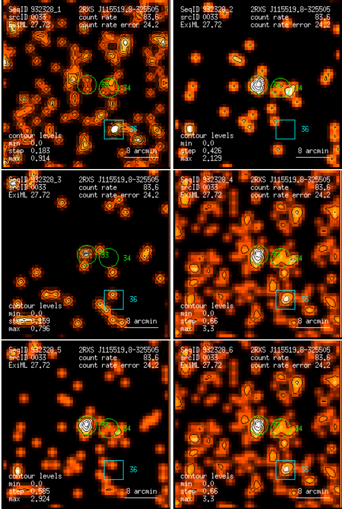
Figure 33: RASS 932328: detection 0033: band rate images, Gaussian filter: (1) PSPC channels 11 – 41, (2) 52 – 90, (3) 91 – 201, (4) 11 – 235, (5) 52 – 201, (6) 11 – 201. Broad band rates in counts/ks. Band rate contour levels in counts/ks/arcmin 2 .
