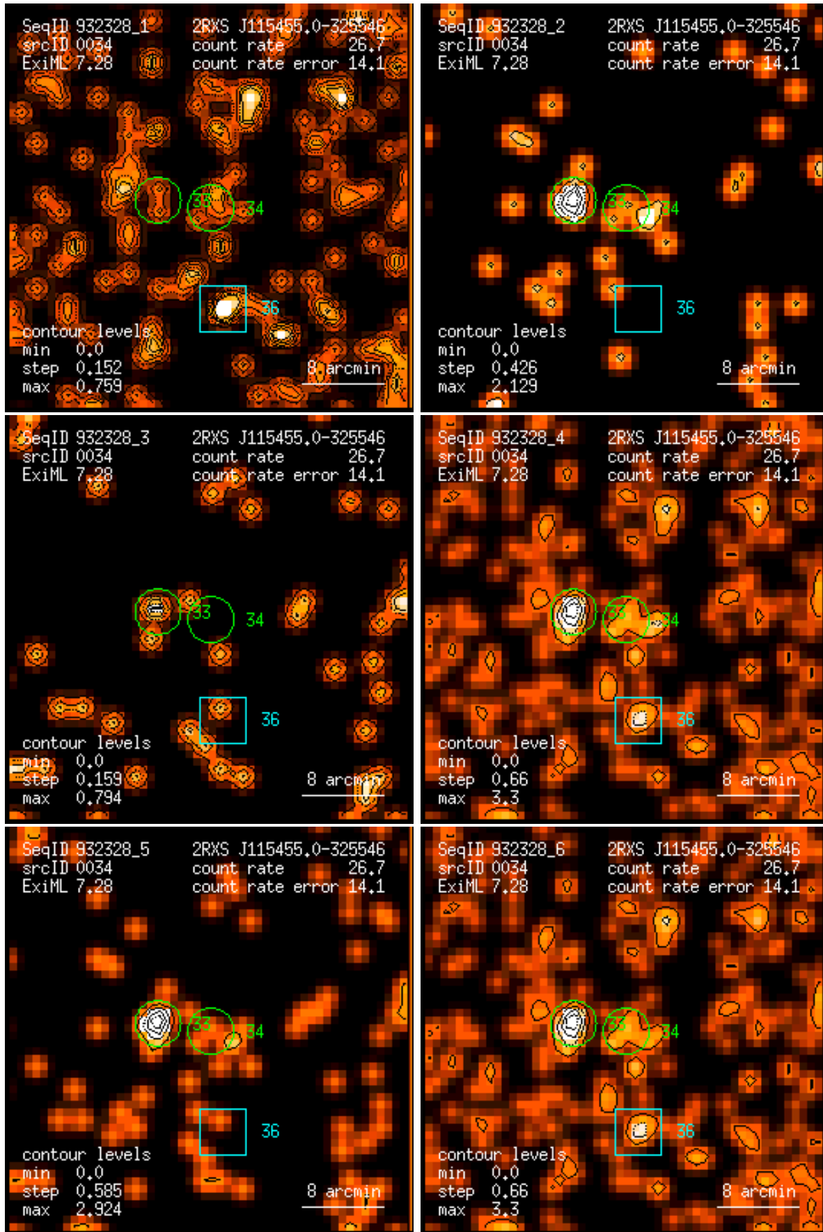
Figure 34: RASS 932328: detection 0034: band rate images, Gaussian filter: (1) PSPC channels 11 – 41, (2) 52 – 90, (3) 91 – 201, (4) 11 – 235, (5) 52 – 201, (6) 11 – 201. Broad band rates in counts/ks. Band rate contour levels in counts/ks/arcmin 2 .
