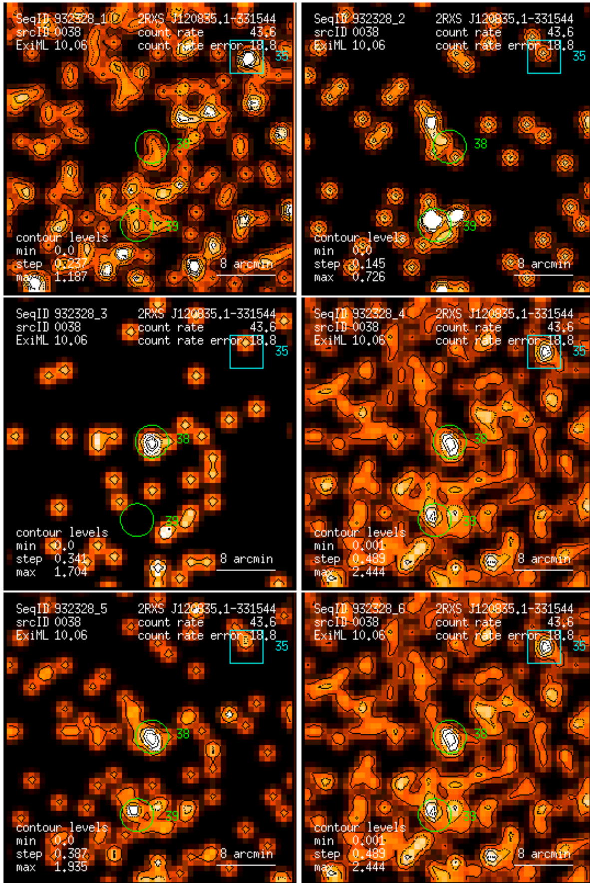
Figure 38: RASS 932328: detection 0038: band rate images, Gaussian filter: (1) PSPC channels 11 – 41, (2) 52 – 90, (3) 91 – 201, (4) 11 – 235, (5) 52 – 201, (6) 11 – 201. Broad band rates in counts/ks. Band rate contour levels in counts/ks/arcmin 2 .
