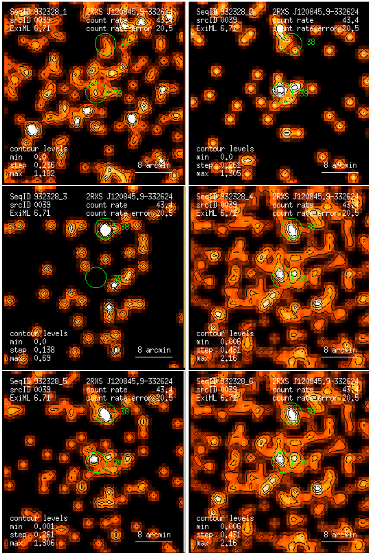
Figure 39: RASS 932328: detection 0039: band rate images, Gaussian filter: (1) PSPC channels 11 – 41, (2) 52 – 90, (3) 91 – 201, (4) 11 – 235, (5) 52 – 201, (6) 11 – 201. Broad band rates in counts/ks. Band rate contour levels in counts/ks/arcmin 2 .
