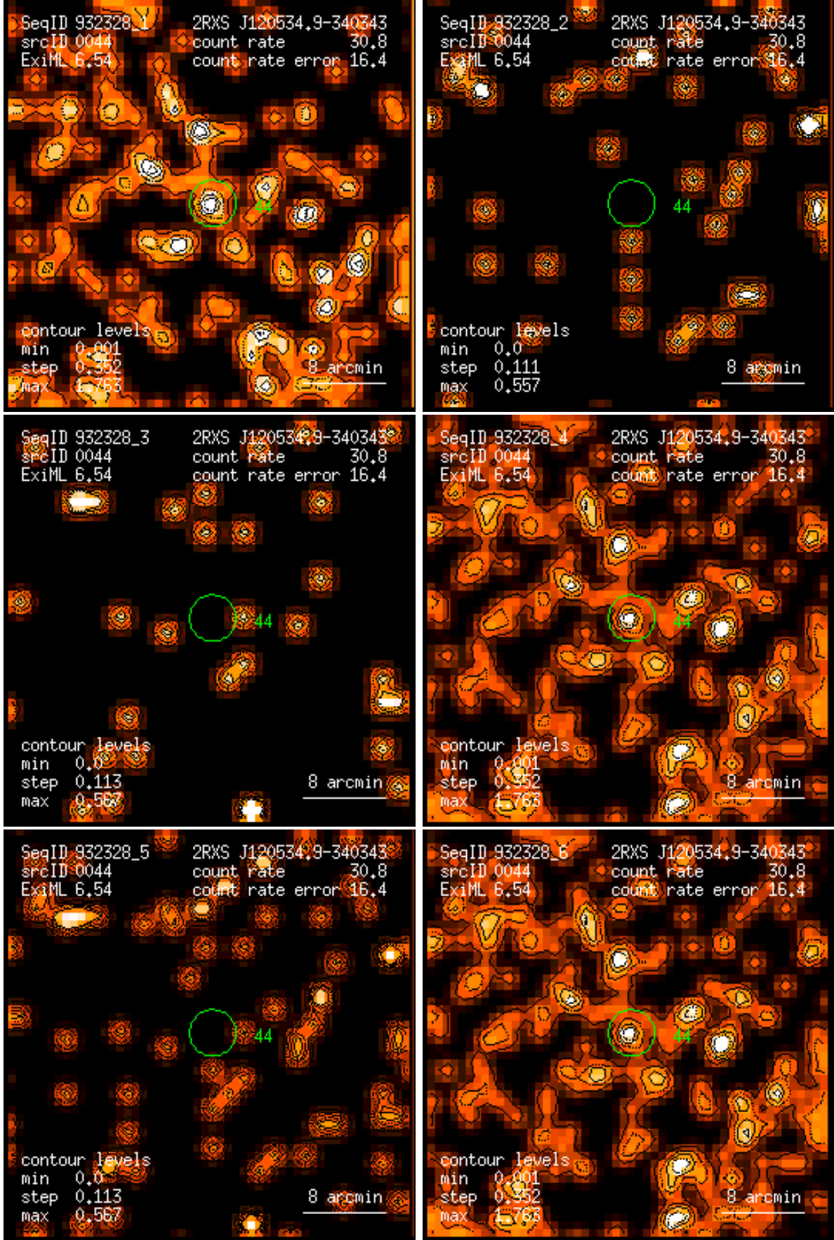
Figure 44: RASS 932328: detection 0044: band rate images, Gaussian filter: (1) PSPC channels 11 – 41, (2) 52 – 90, (3) 91 – 201, (4) 11 – 235, (5) 52 – 201, (6) 11 – 201. Broad band rates in counts/ks. Band rate contour levels in counts/ks/arcmin 2 .
