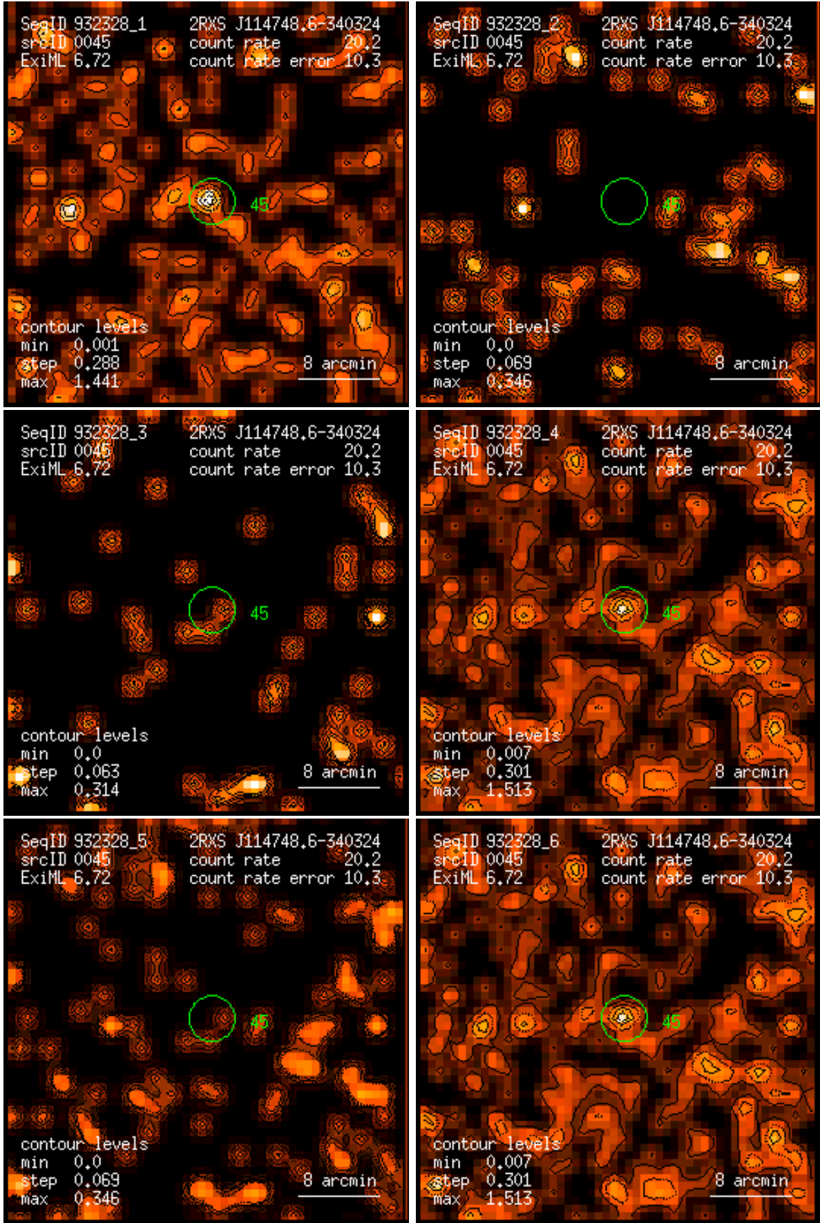
Figure 45: RASS 932328: detection 0045: band rate images, Gaussian filter: (1) PSPC channels 11 – 41, (2) 52 – 90, (3) 91 – 201, (4) 11 – 235, (5) 52 – 201, (6) 11 – 201. Broad band rates in counts/ks. Band rate contour levels in counts/ks/arcmin 2 .
