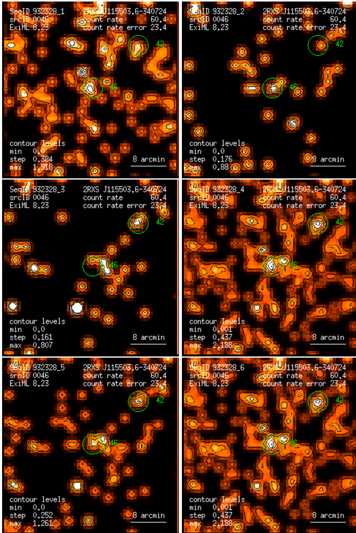
Figure 46: RASS 932328: detection 0046: band rate images, Gaussian filter: (1) PSPC channels 11 – 41, (2) 52 – 90, (3) 91 – 201, (4) 11 – 235, (5) 52 – 201, (6) 11 – 201. Broad band rates in counts/ks. Band rate contour levels in counts/ks/arcmin 2 .
