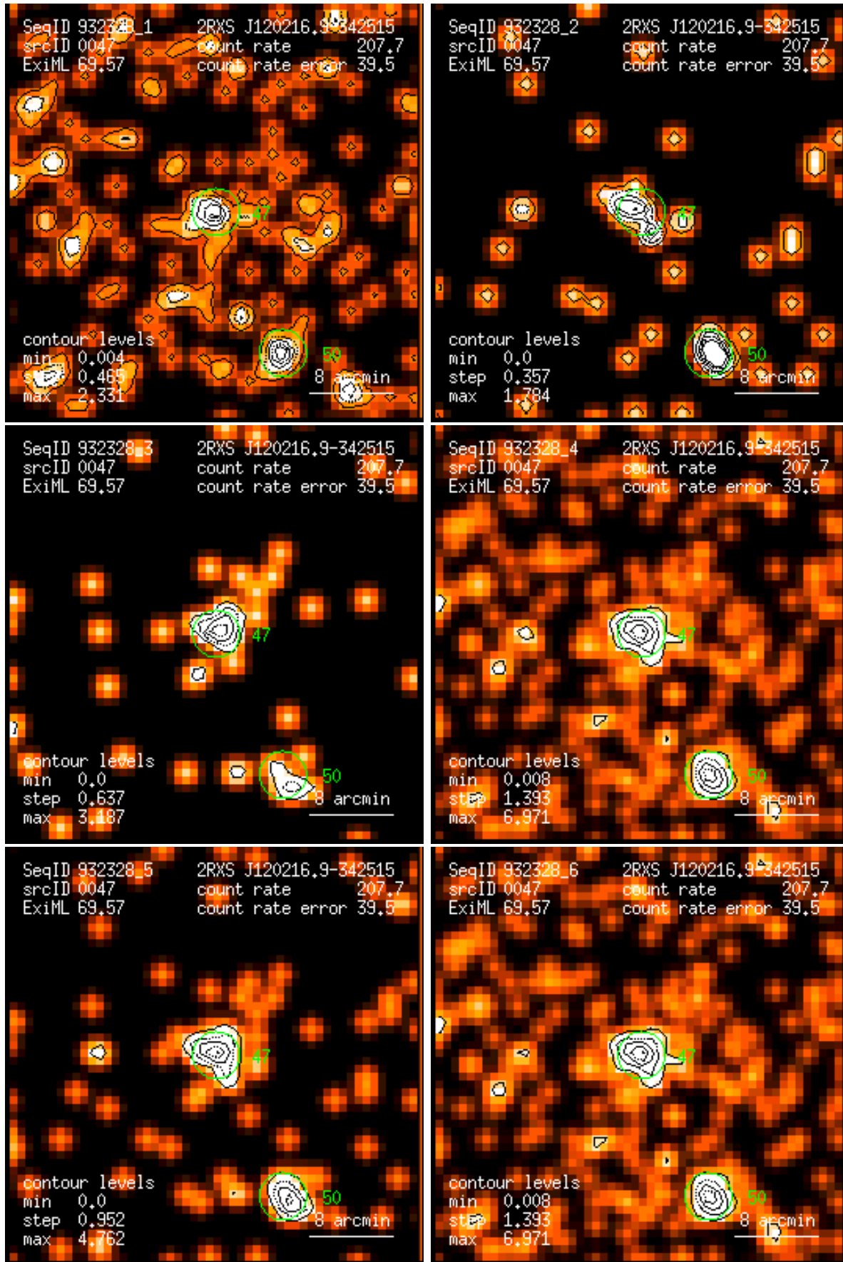
Figure 47: RASS 932328: detection 0047: band rate images, Gaussian filter: (1) PSPC channels 11 – 41, (2) 52 – 90, (3) 91 – 201, (4) 11 – 235, (5) 52 – 201, (6) 11 – 201. Broad band rates in counts/ks. Band rate contour levels in counts/ks/arcmin 2 .
