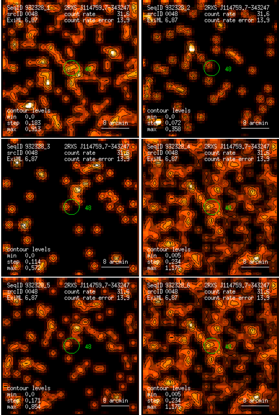
Figure 48: RASS 932328: detection 0048: band rate images, Gaussian filter: (1) PSPC channels 11 – 41, (2) 52 – 90, (3) 91 – 201, (4) 11 – 235, (5) 52 – 201, (6) 11 – 201. Broad band rates in counts/ks. Band rate contour levels in counts/ks/arcmin 2 .
