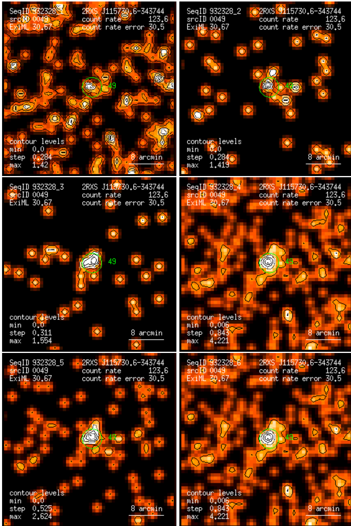
Figure 49: RASS 932328: detection 0049: band rate images, Gaussian filter: (1) PSPC channels 11 – 41, (2) 52 – 90, (3) 91 – 201, (4) 11 – 235, (5) 52 – 201, (6) 11 – 201. Broad band rates in counts/ks. Band rate contour levels in counts/ks/arcmin 2 .
