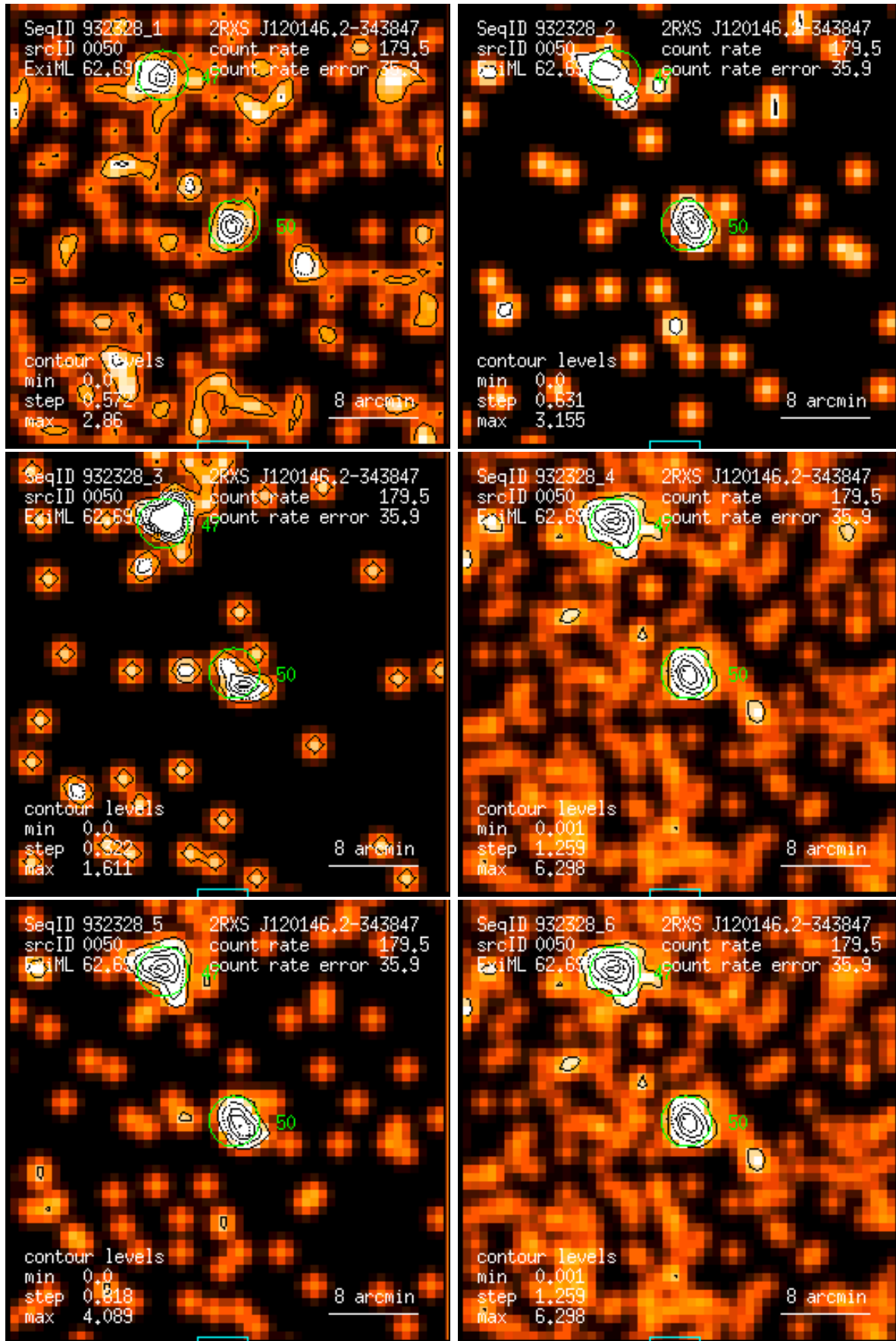
Figure 50: RASS 932328: detection 0050: band rate images, Gaussian filter: (1) PSPC channels 11 – 41, (2) 52 – 90, (3) 91 – 201, (4) 11 – 235, (5) 52 – 201, (6) 11 – 201. Broad band rates in counts/ks. Band rate contour levels in counts/ks/arcmin 2 .
