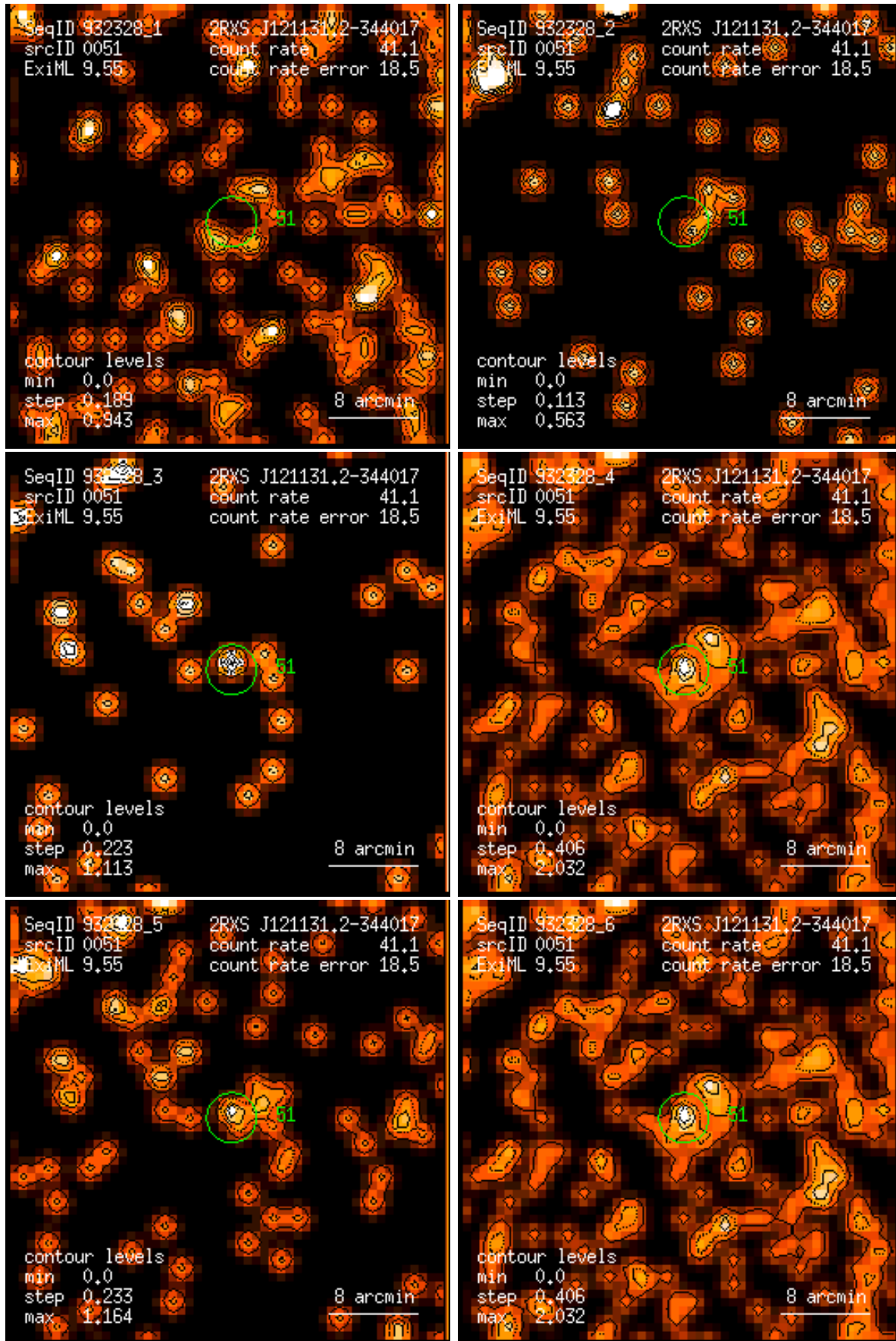
Figure 51: RASS 932328: detection 0051: band rate images, Gaussian filter: (1) PSPC channels 11 – 41, (2) 52 – 90, (3) 91 – 201, (4) 11 – 235, (5) 52 – 201, (6) 11 – 201. Broad band rates in counts/ks. Band rate contour levels in counts/ks/arcmin 2 .
