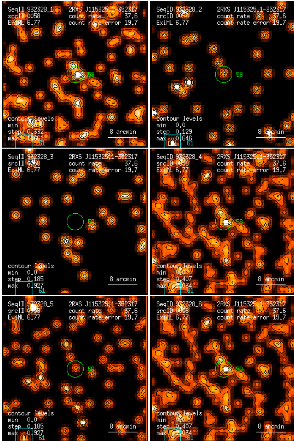
Figure 58: RASS 932328: detection 0058: band rate images, Gaussian filter: (1) PSPC channels 11 – 41, (2) 52 – 90, (3) 91 – 201, (4) 11 – 235, (5) 52 – 201, (6) 11 – 201. Broad band rates in counts/ks. Band rate contour levels in counts/ks/arcmin 2 .
