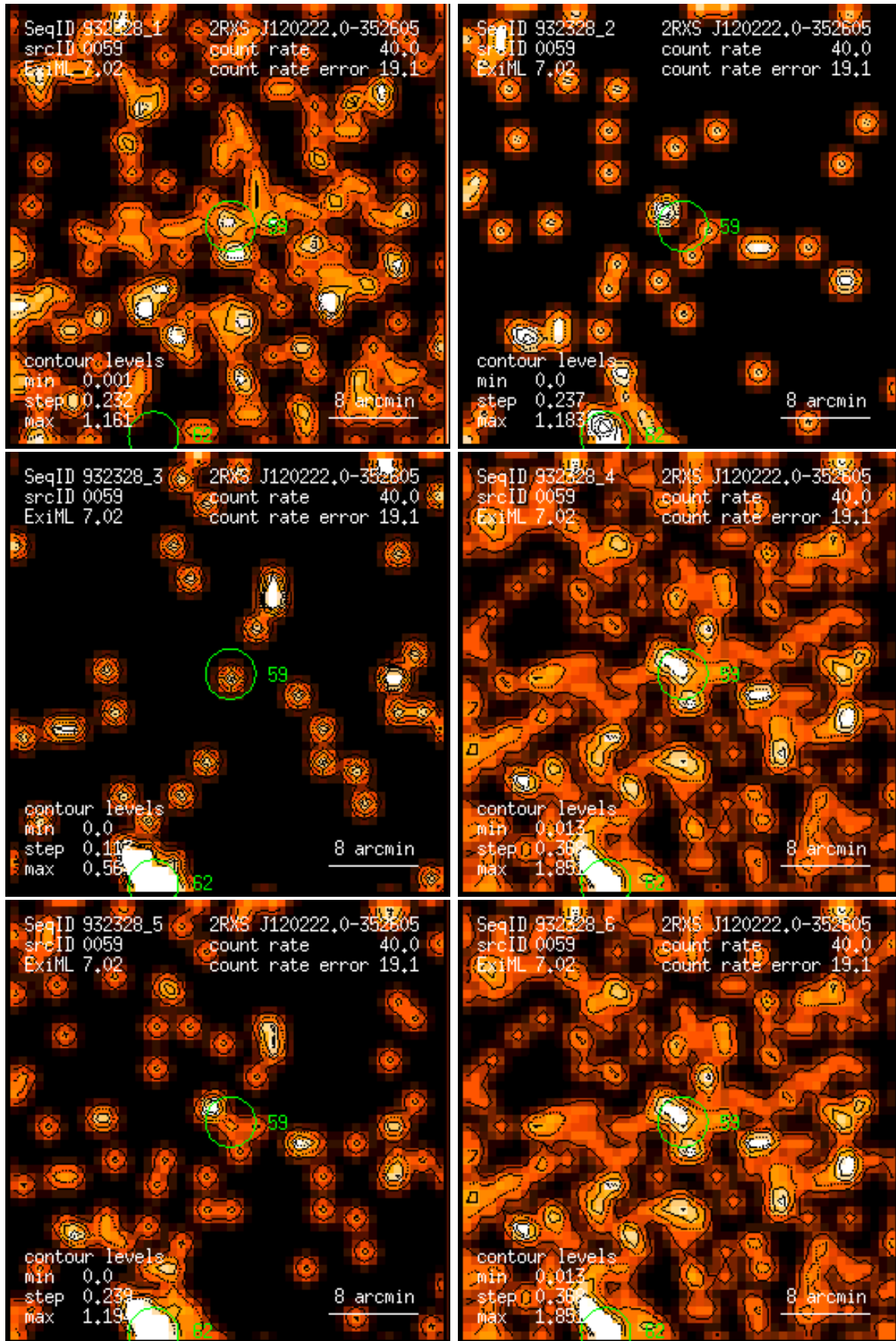
Figure 59: RASS 932328: detection 0059: band rate images, Gaussian filter: (1) PSPC channels 11 – 41, (2) 52 – 90, (3) 91 – 201, (4) 11 – 235, (5) 52 – 201, (6) 11 – 201. Broad band rates in counts/ks. Band rate contour levels in counts/ks/arcmin 2 .
