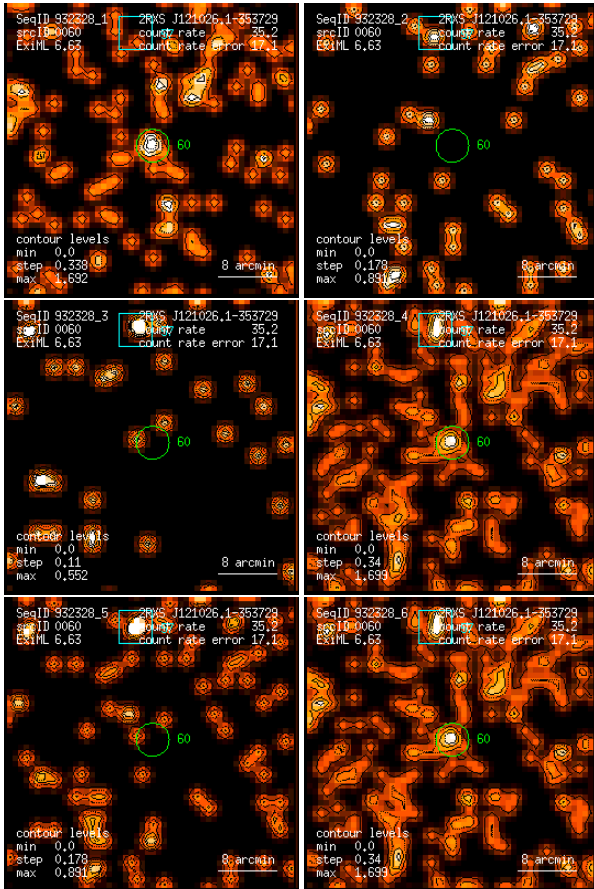
Figure 60: RASS 932328: detection 0060: band rate images, Gaussian filter: (1) PSPC channels 11 – 41, (2) 52 – 90, (3) 91 – 201, (4) 11 – 235, (5) 52 – 201, (6) 11 – 201. Broad band rates in counts/ks. Band rate contour levels in counts/ks/arcmin 2 .
