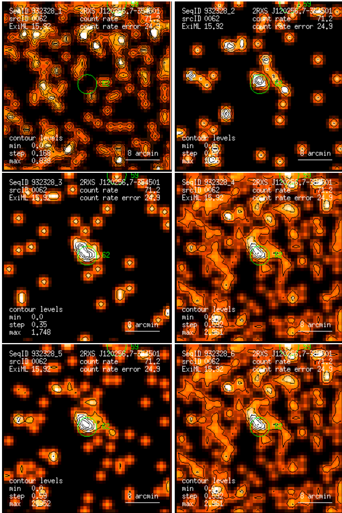
Figure 62: RASS 932328: detection 0062: band rate images, Gaussian filter: (1) PSPC channels 11 – 41, (2) 52 – 90, (3) 91 – 201, (4) 11 – 235, (5) 52 – 201, (6) 11 – 201. Broad band rates in counts/ks. Band rate contour levels in counts/ks/arcmin 2 .
