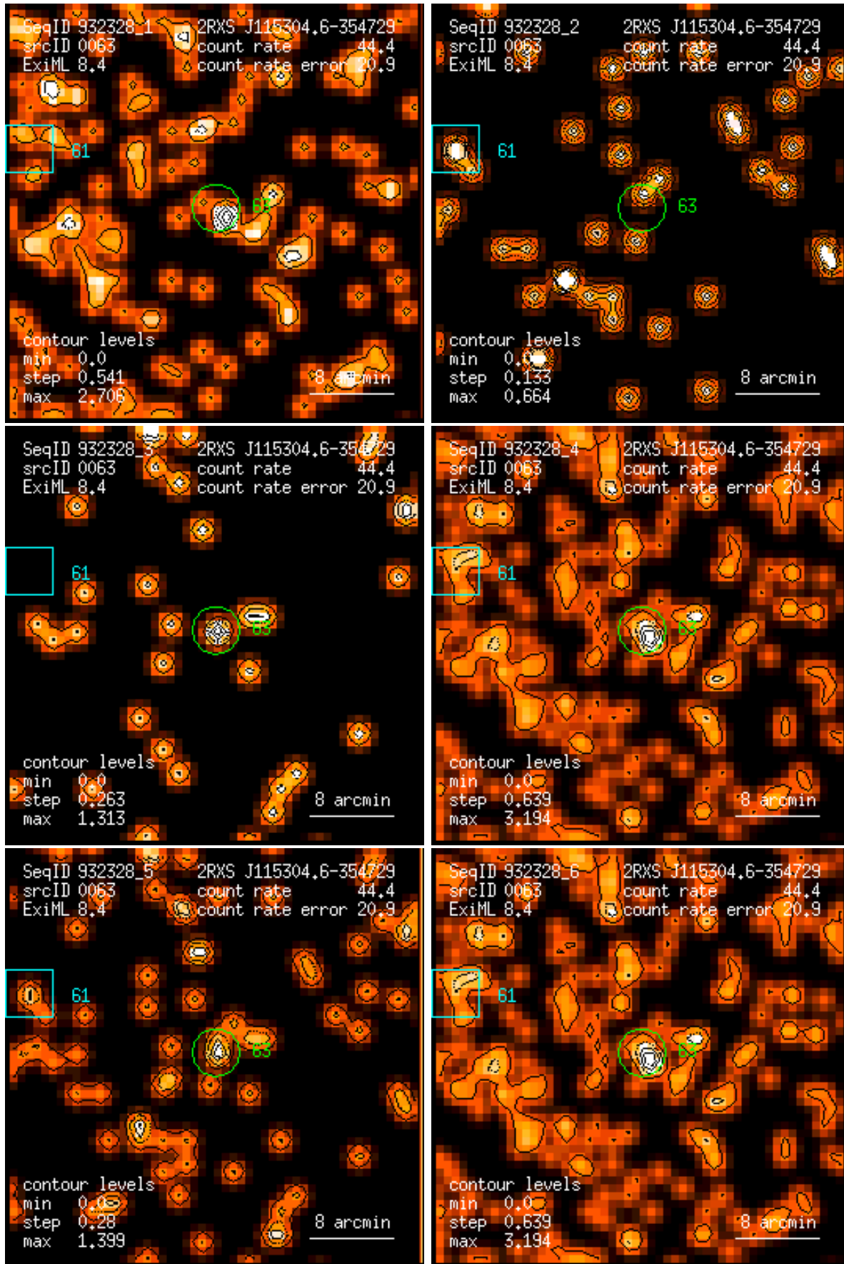
Figure 63: RASS 932328: detection 0063: band rate images, Gaussian filter: (1) PSPC channels 11 – 41, (2) 52 – 90, (3) 91 – 201, (4) 11 – 235, (5) 52 – 201, (6) 11 – 201. Broad band rates in counts/ks. Band rate contour levels in counts/ks/arcmin 2 .
