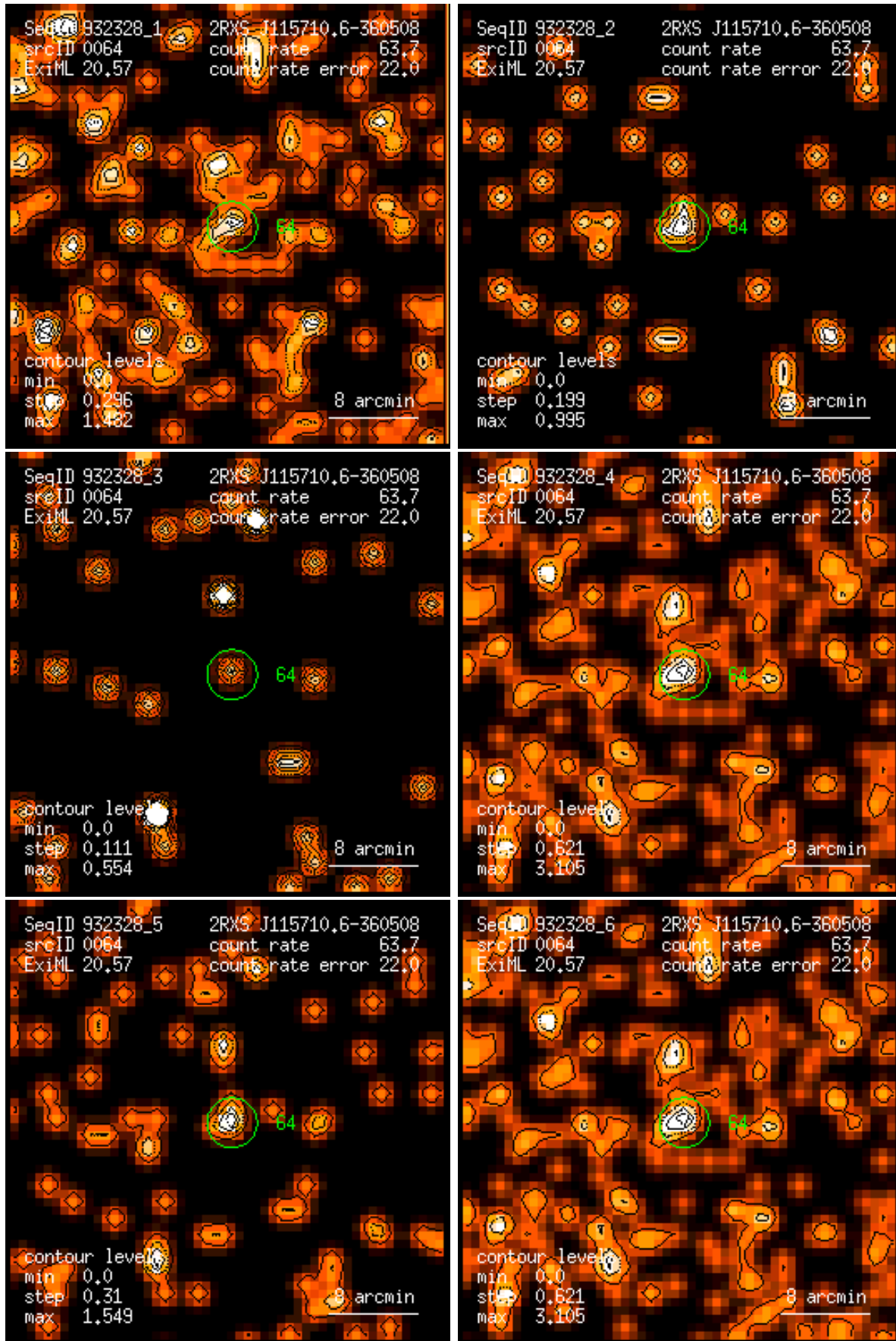
Figure 64: RASS 932328: detection 0064: band rate images, Gaussian filter: (1) PSPC channels 11 – 41, (2) 52 – 90, (3) 91 – 201, (4) 11 – 235, (5) 52 – 201, (6) 11 – 201. Broad band rates in counts/ks. Band rate contour levels in counts/ks/arcmin 2 .
