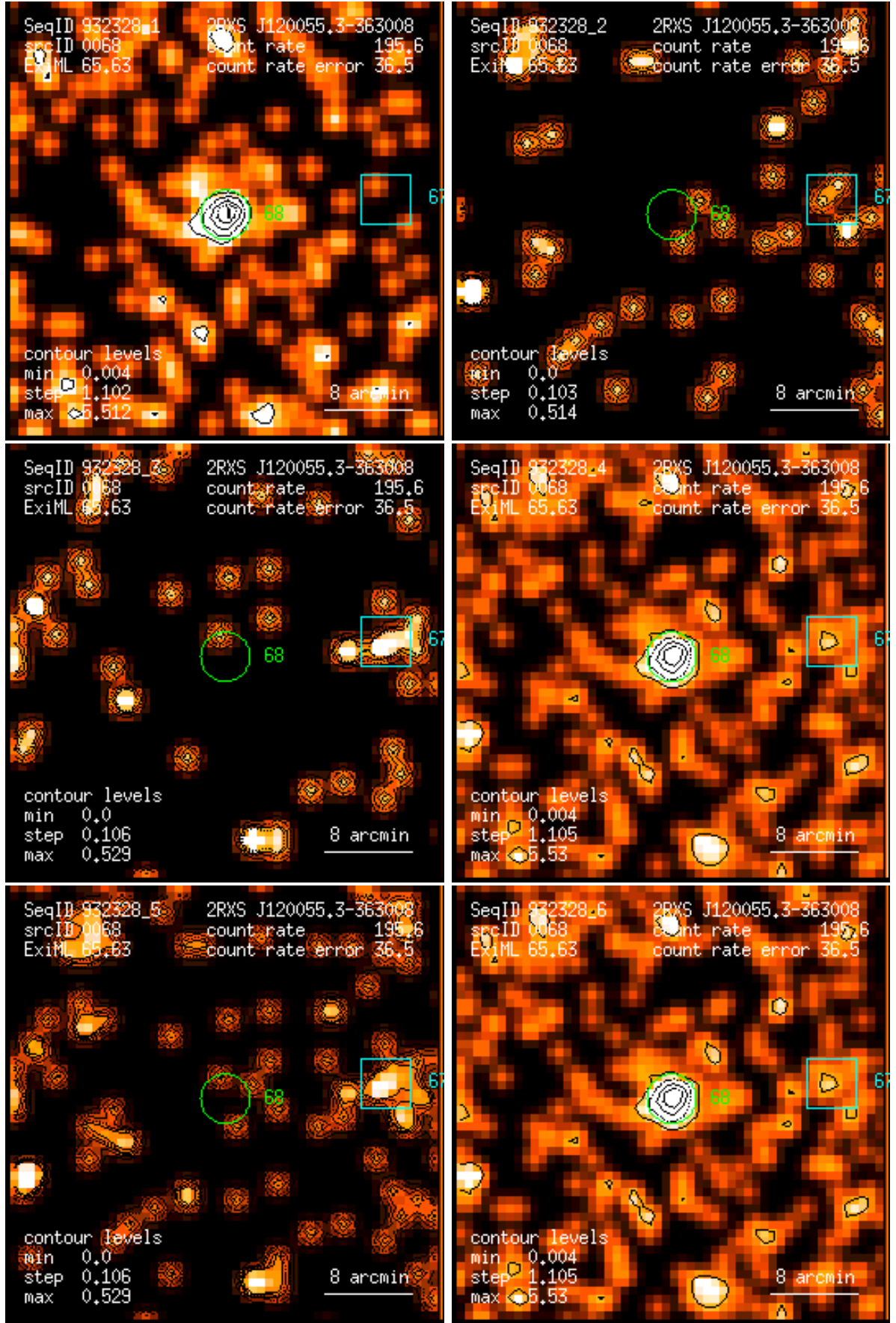
Figure 68: RASS 932328: detection 0068: band rate images, Gaussian filter: (1) PSPC channels 11 – 41, (2) 52 – 90, (3) 91 – 201, (4) 11 – 235, (5) 52 – 201, (6) 11 – 201. Broad band rates in counts/ks. Band rate contour levels in counts/ks/arcmin 2 .
