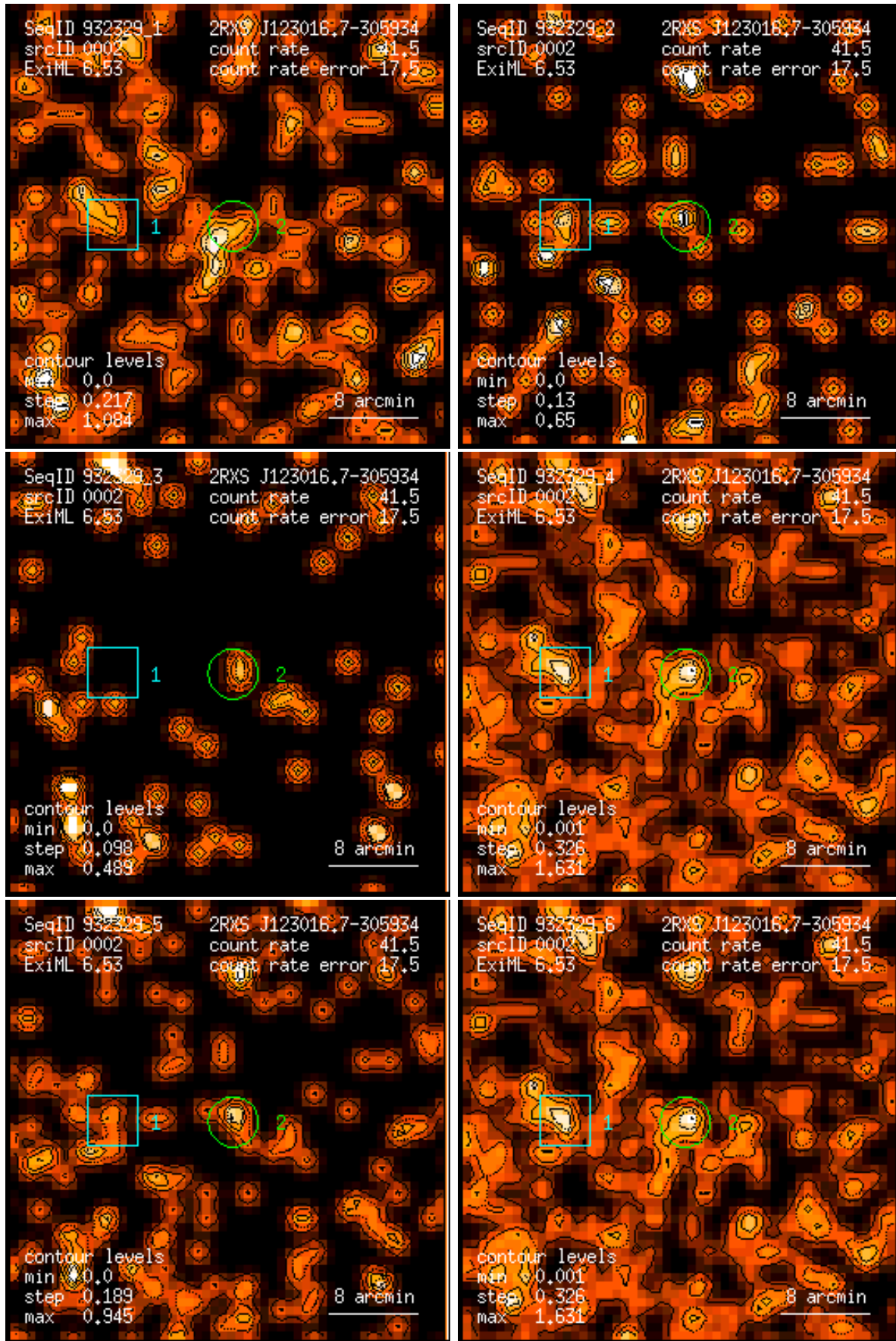
Figure 2: RASS 932329: detection 0002: band rate images, Gaussian filter: (1) PSPC channels 11 – 41, (2) 52 – 90, (3) 91 – 201, (4) 11 – 235, (5) 52 – 201, (6) 11 – 201. Broad band rates in counts/ks. Band rate contour levels in counts/ks/arcmin 2 .
