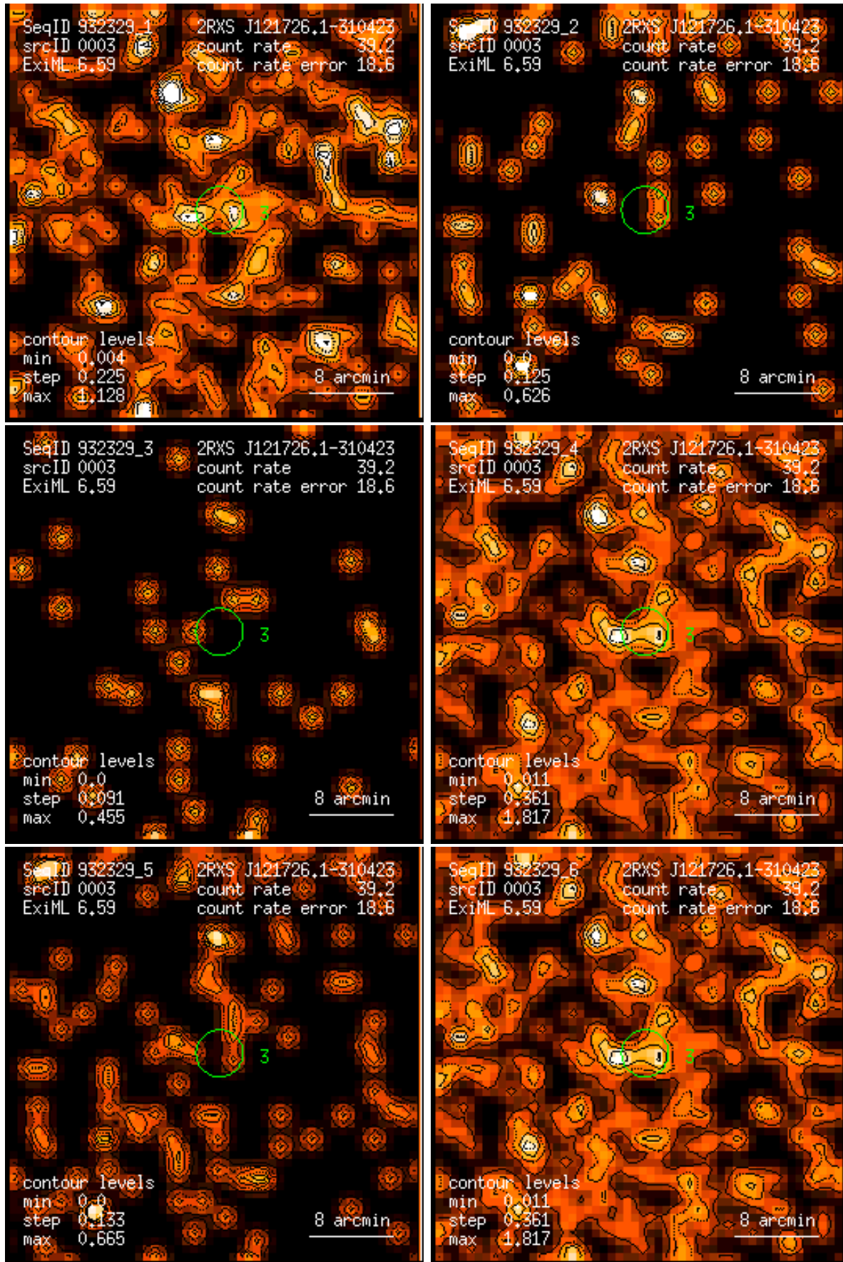
Figure 3: RASS 932329: detection 0003: band rate images, Gaussian filter: (1) PSPC channels 11 – 41, (2) 52 – 90, (3) 91 – 201, (4) 11 – 235, (5) 52 – 201, (6) 11 – 201. Broad band rates in counts/ks. Band rate contour levels in counts/ks/arcmin 2 .
