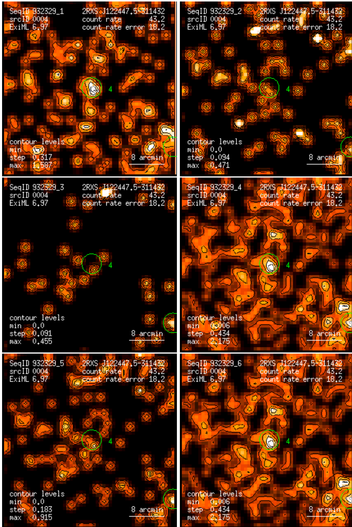
Figure 4: RASS 932329: detection 0004: band rate images, Gaussian filter: (1) PSPC channels 11 – 41, (2) 52 – 90, (3) 91 – 201, (4) 11 – 235, (5) 52 – 201, (6) 11 – 201. Broad band rates in counts/ks. Band rate contour levels in counts/ks/arcmin 2 .
