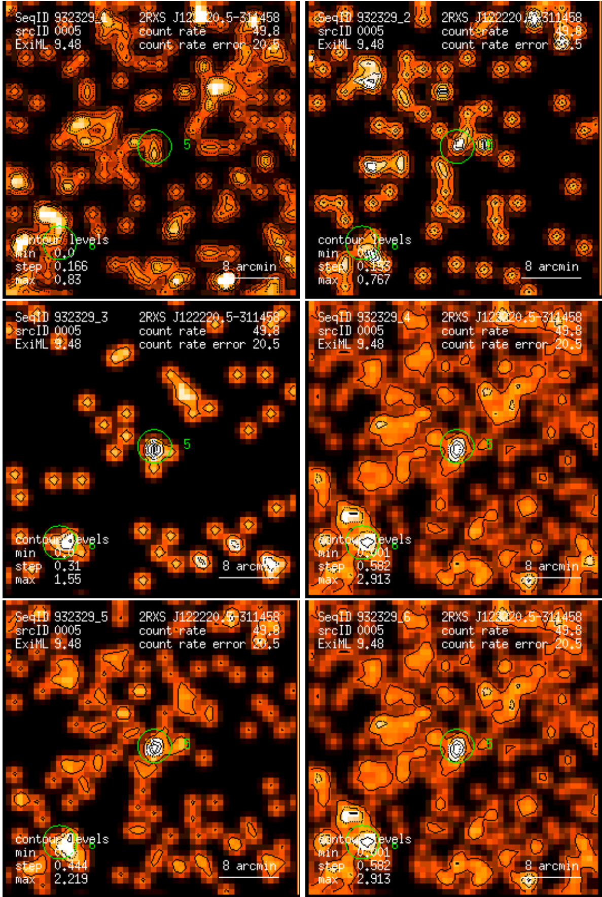
Figure 5: RASS 932329: detection 0005: band rate images, Gaussian filter: (1) PSPC channels 11 – 41, (2) 52 – 90, (3) 91 – 201, (4) 11 – 235, (5) 52 – 201, (6) 11 – 201. Broad band rates in counts/ks. Band rate contour levels in counts/ks/arcmin 2 .
