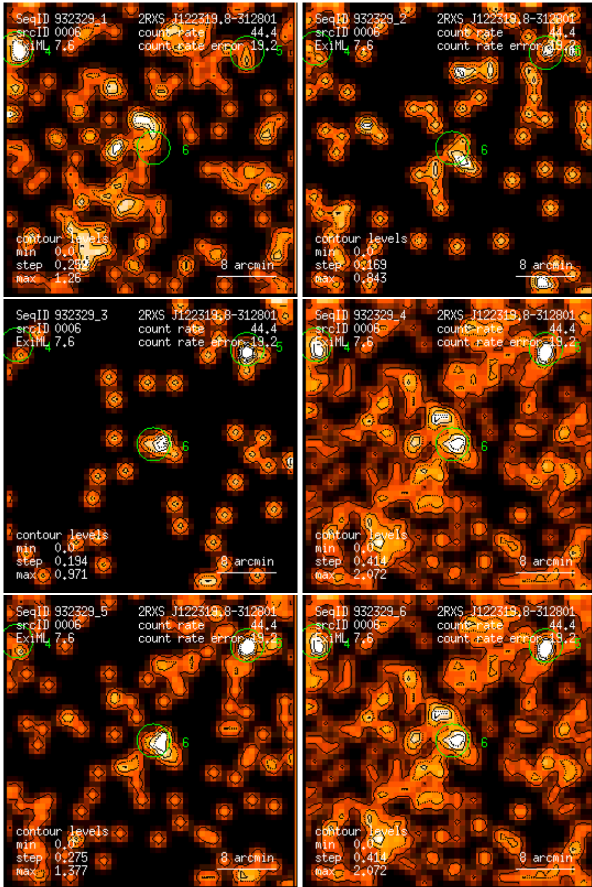
Figure 6: RASS 932329: detection 0006: band rate images, Gaussian filter: (1) PSPC channels 11 – 41, (2) 52 – 90, (3) 91 – 201, (4) 11 – 235, (5) 52 – 201, (6) 11 – 201. Broad band rates in counts/ks. Band rate contour levels in counts/ks/arcmin 2 .
