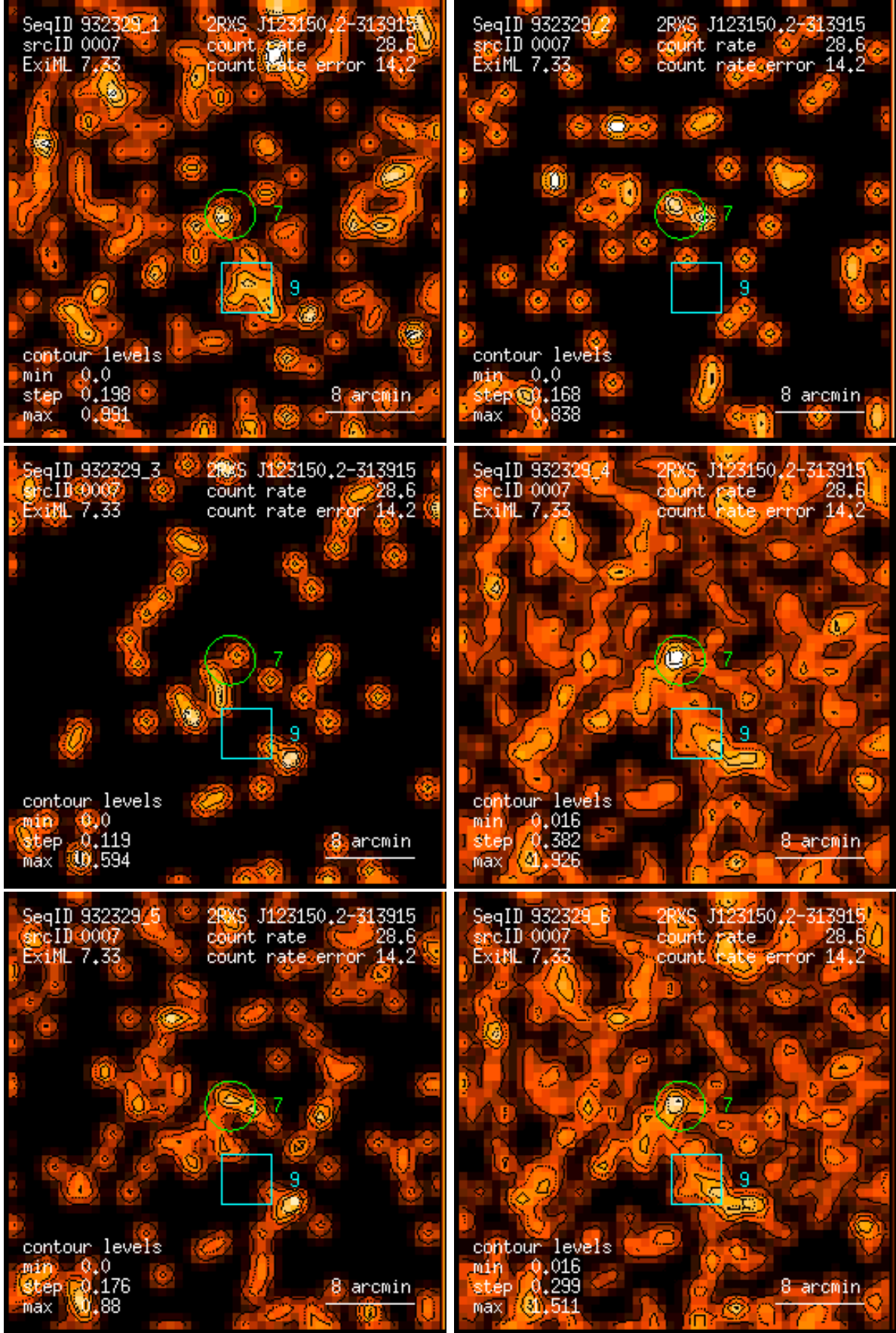
Figure 7: RASS 932329: detection 0007: band rate images, Gaussian filter: (1) PSPC channels 11 – 41, (2) 52 – 90, (3) 91 – 201, (4) 11 – 235, (5) 52 – 201, (6) 11 – 201. Broad band rates in counts/ks. Band rate contour levels in counts/ks/arcmin 2 .
