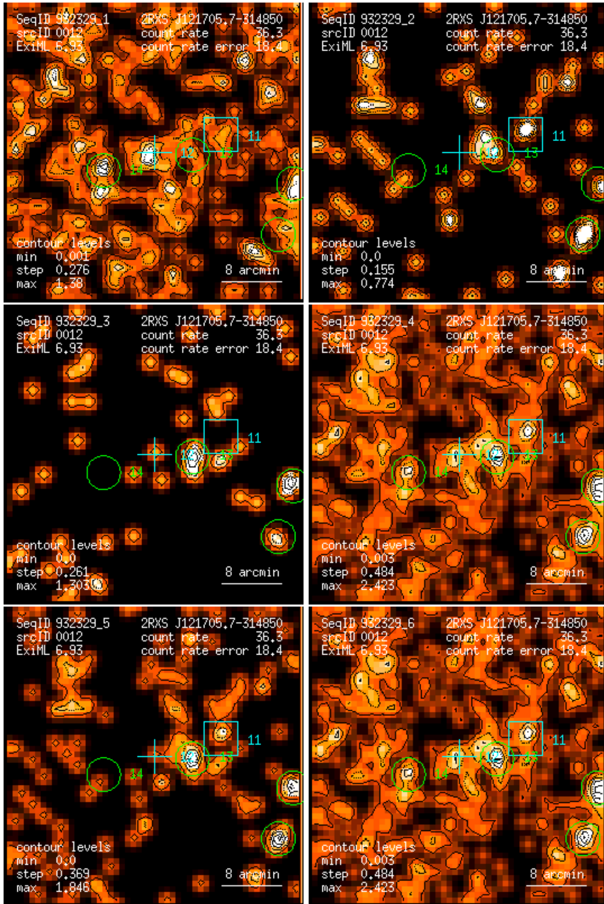
Figure 12: RASS 932329: detection 0012: band rate images, Gaussian filter: (1) PSPC channels 11 – 41, (2) 52 – 90, (3) 91 – 201, (4) 11 – 235, (5) 52 – 201, (6) 11 – 201. Broad band rates in counts/ks. Band rate contour levels in counts/ks/arcmin 2 .
