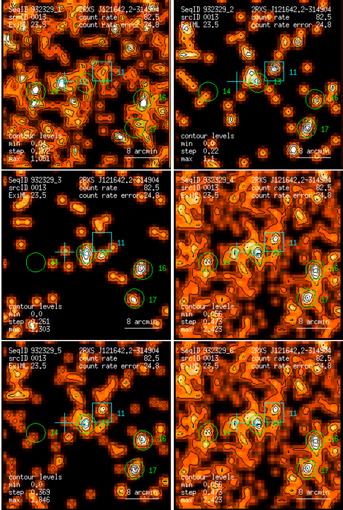
Figure 13: RASS 932329: detection 0013: band rate images, Gaussian filter: (1) PSPC channels 11 – 41, (2) 52 – 90, (3) 91 – 201, (4) 11 – 235, (5) 52 – 201, (6) 11 – 201. Broad band rates in counts/ks. Band rate contour levels in counts/ks/arcmin 2 .
