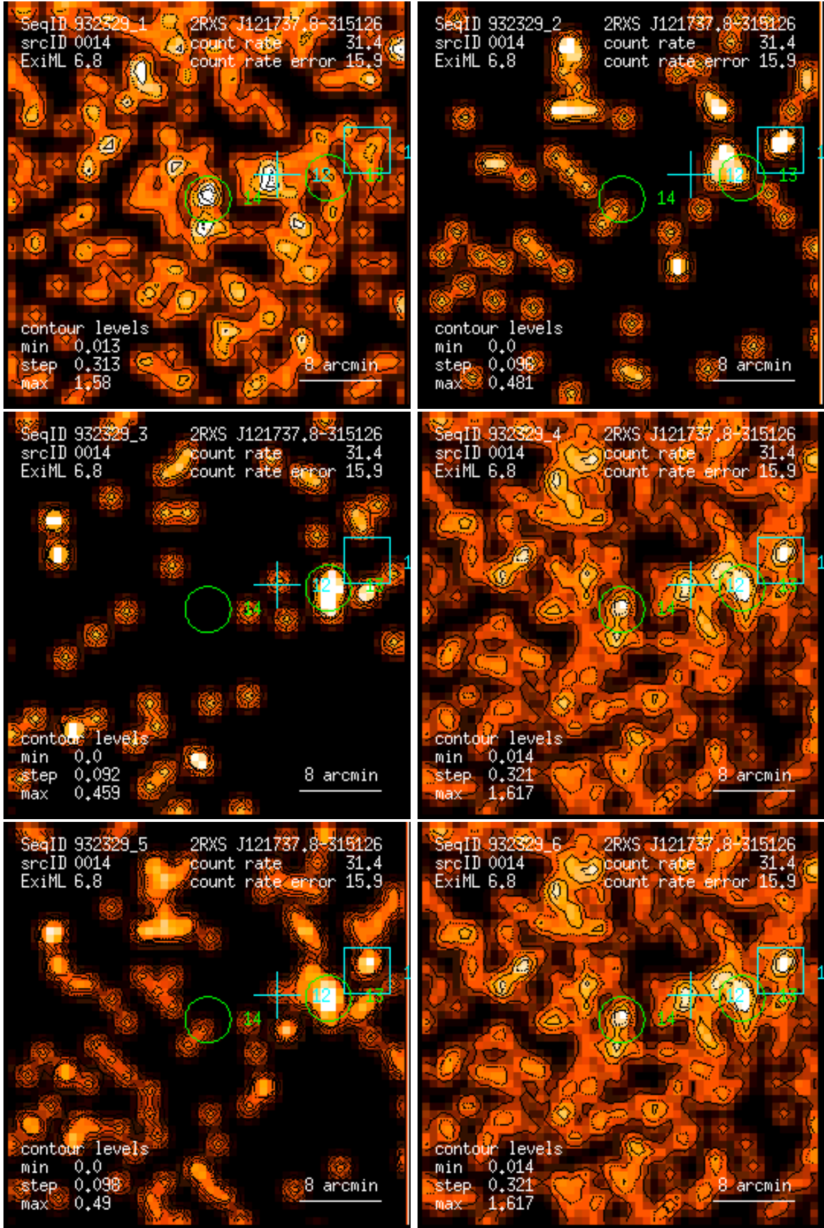
Figure 14: RASS 932329: detection 0014: band rate images, Gaussian filter: (1) PSPC channels 11 – 41, (2) 52 – 90, (3) 91 – 201, (4) 11 – 235, (5) 52 – 201, (6) 11 – 201. Broad band rates in counts/ks. Band rate contour levels in counts/ks/arcmin 2 .
