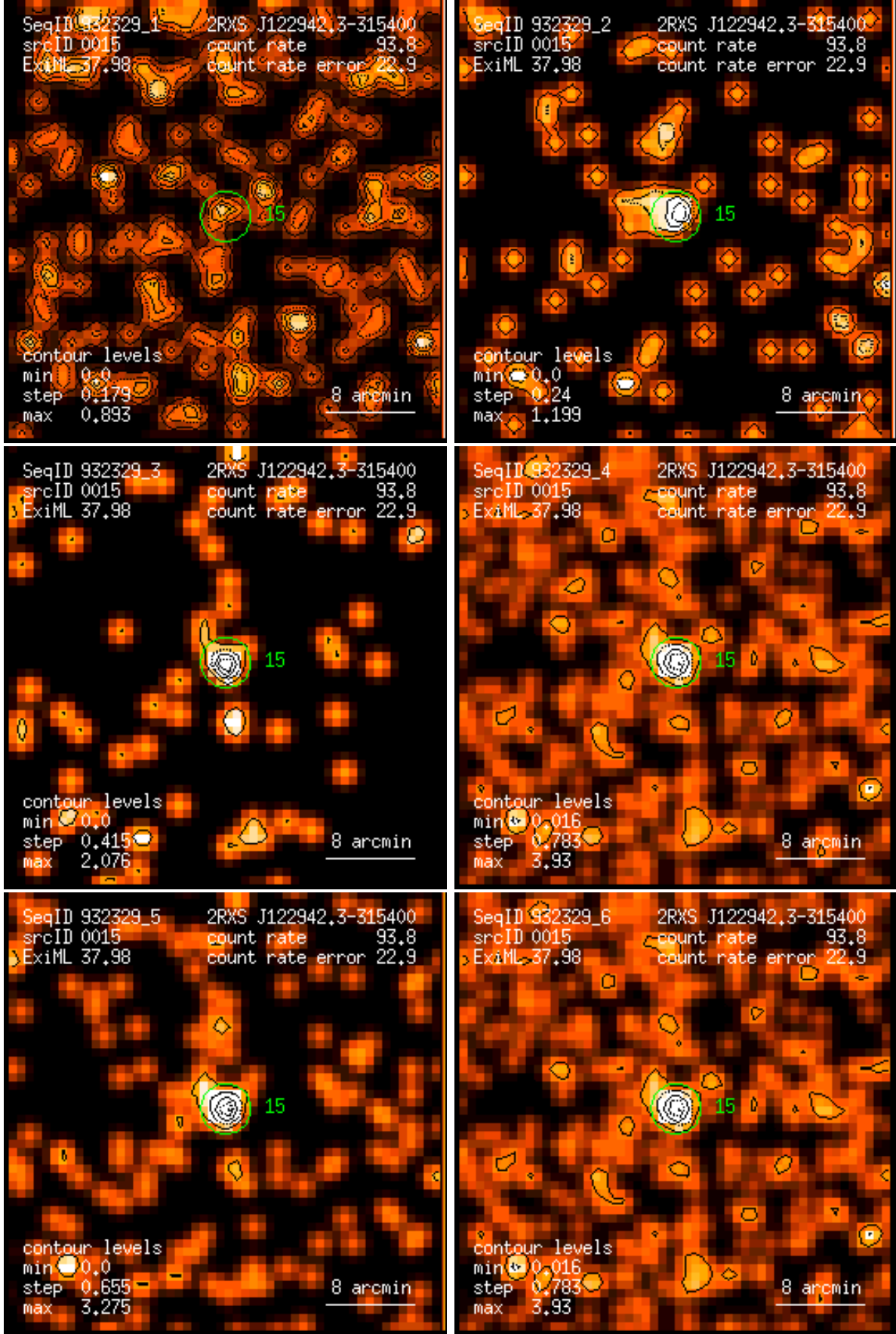
Figure 15: RASS 932329: detection 0015: band rate images, Gaussian filter: (1) PSPC channels 11 – 41, (2) 52 – 90, (3) 91 – 201, (4) 11 – 235, (5) 52 – 201, (6) 11 – 201. Broad band rates in counts/ks. Band rate contour levels in counts/ks/arcmin 2 .
