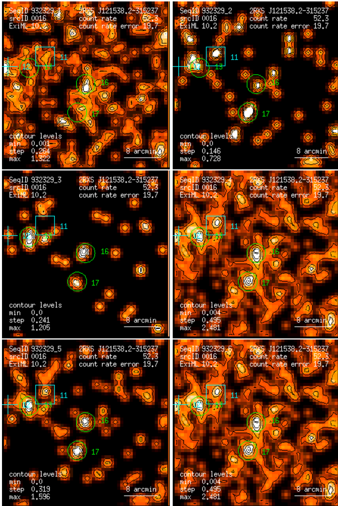
Figure 16: RASS 932329: detection 0016: band rate images, Gaussian filter: (1) PSPC channels 11 – 41, (2) 52 – 90, (3) 91 – 201, (4) 11 – 235, (5) 52 – 201, (6) 11 – 201. Broad band rates in counts/ks. Band rate contour levels in counts/ks/arcmin 2 .
