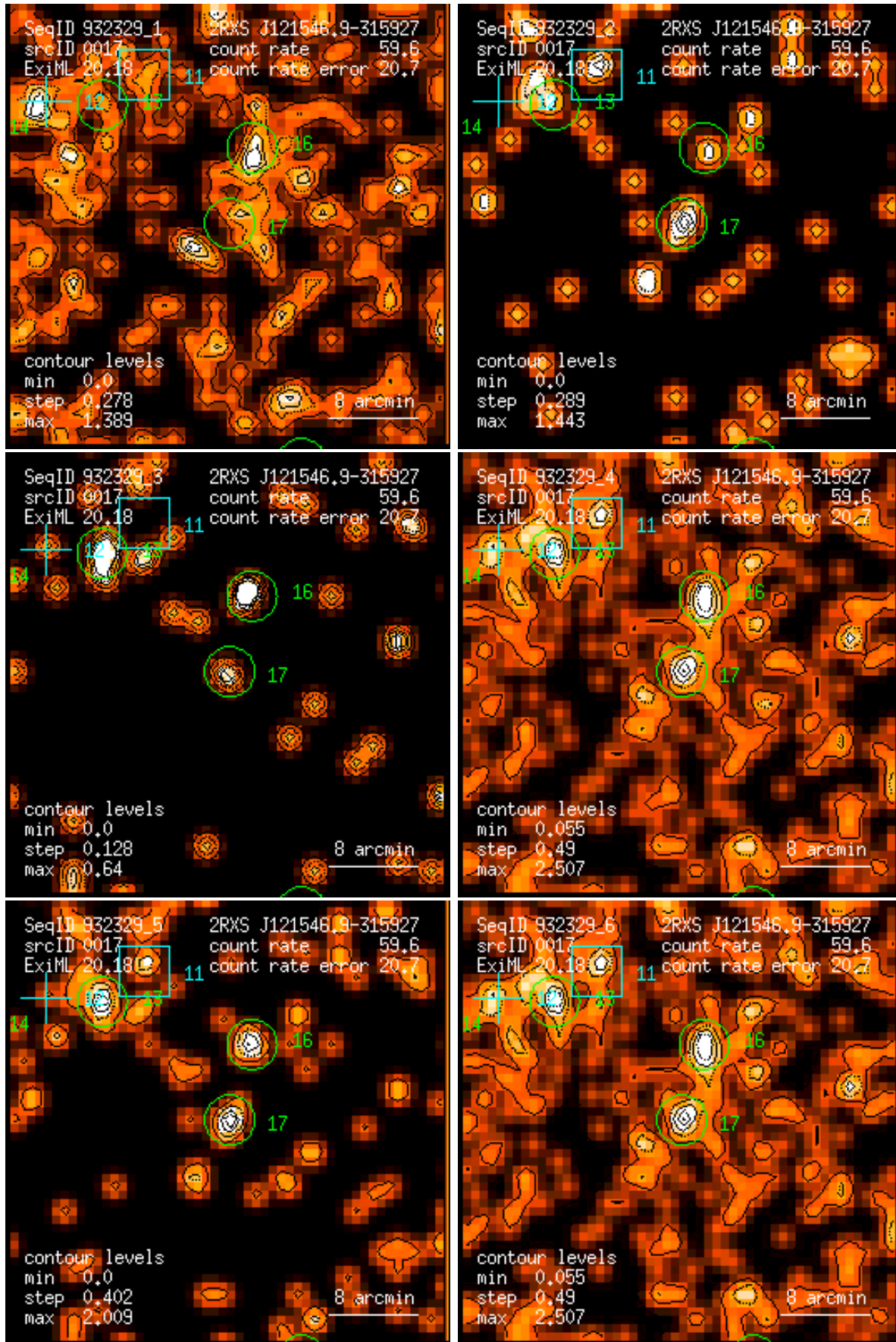
Figure 17: RASS 932329: detection 0017: band rate images, Gaussian filter: (1) PSPC channels 11 – 41, (2) 52 – 90, (3) 91 – 201, (4) 11 – 235, (5) 52 – 201, (6) 11 – 201. Broad band rates in counts/ks. Band rate contour levels in counts/ks/arcmin 2 .
