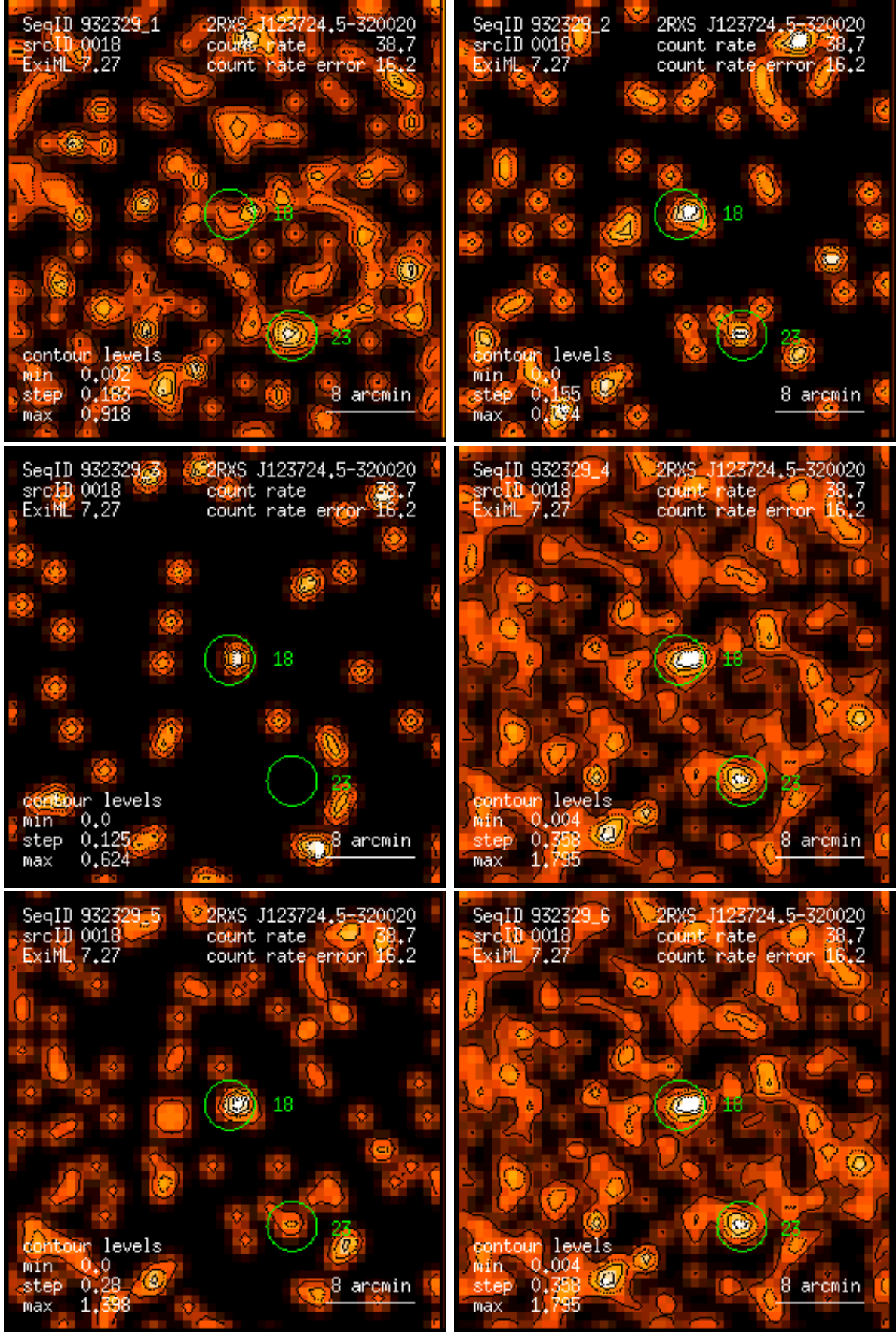
Figure 18: RASS 932329: detection 0018: band rate images, Gaussian filter: (1) PSPC channels 11 – 41, (2) 52 – 90, (3) 91 – 201, (4) 11 – 235, (5) 52 – 201, (6) 11 – 201. Broad band rates in counts/ks. Band rate contour levels in counts/ks/arcmin 2 .
