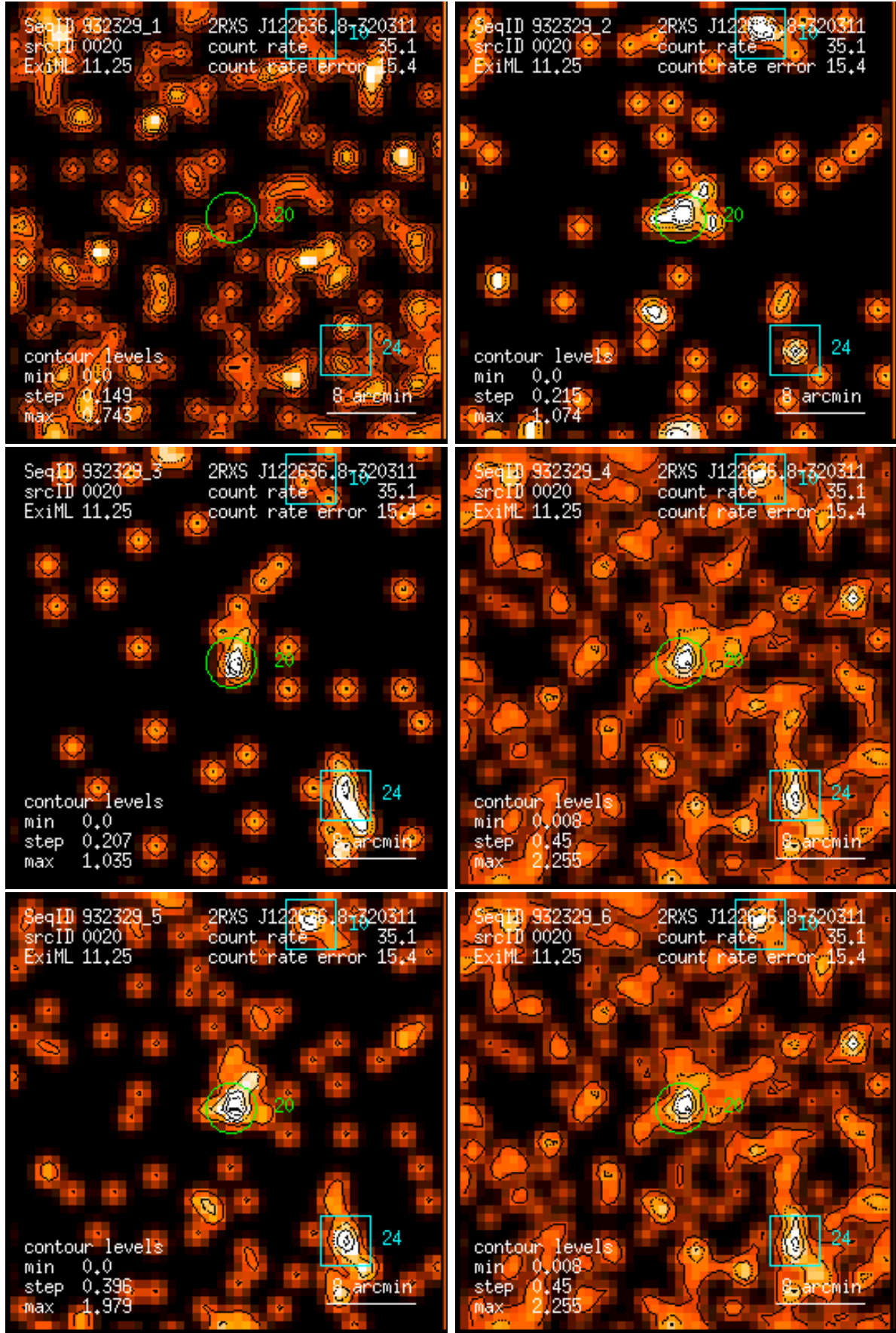
Figure 20: RASS 932329: detection 0020: band rate images, Gaussian filter: (1) PSPC channels 11 – 41, (2) 52 – 90, (3) 91 – 201, (4) 11 – 235, (5) 52 – 201, (6) 11 – 201. Broad band rates in counts/ks. Band rate contour levels in counts/ks/arcmin 2 .
