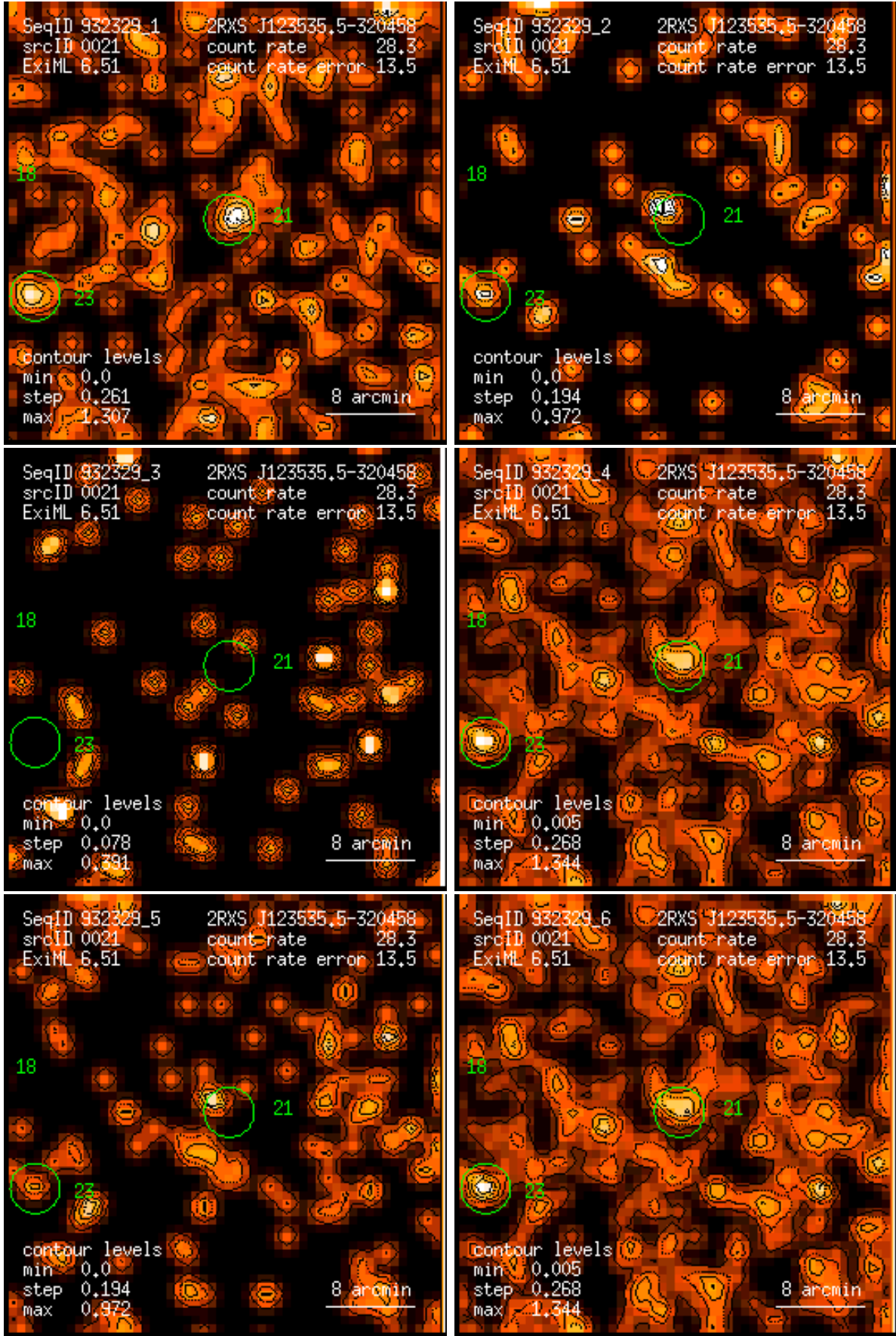
Figure 21: RASS 932329: detection 0021: band rate images, Gaussian filter: (1) PSPC channels 11 – 41, (2) 52 – 90, (3) 91 – 201, (4) 11 – 235, (5) 52 – 201, (6) 11 – 201. Broad band rates in counts/ks. Band rate contour levels in counts/ks/arcmin 2 .
