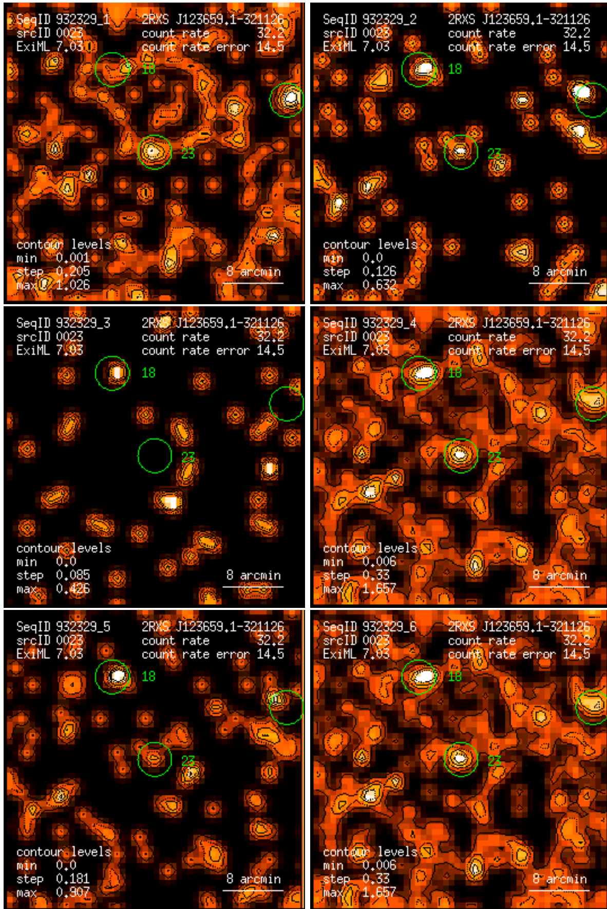
Figure 23: RASS 932329: detection 0023: band rate images, Gaussian filter: (1) PSPC channels 11 – 41, (2) 52 – 90, (3) 91 – 201, (4) 11 – 235, (5) 52 – 201, (6) 11 – 201. Broad band rates in counts/ks. Band rate contour levels in counts/ks/arcmin 2 .
