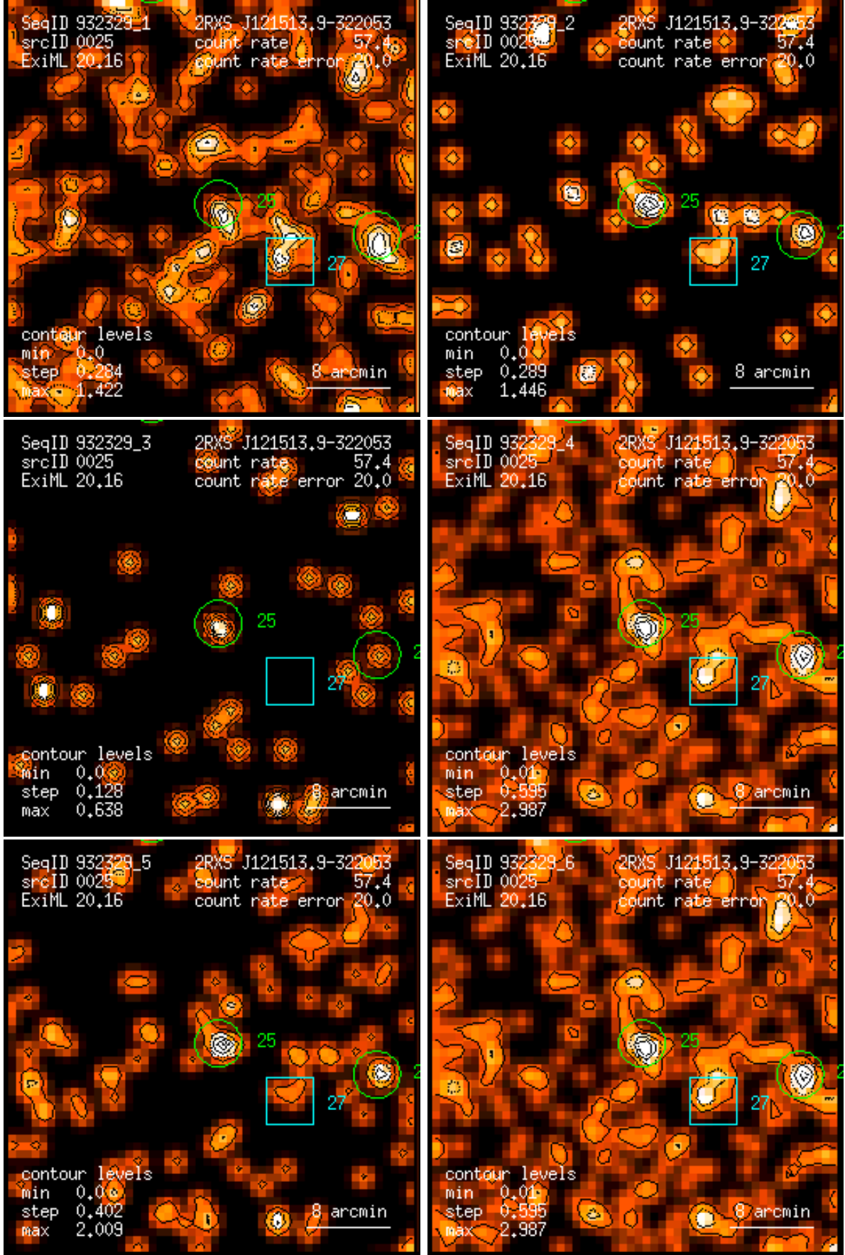
Figure 25: RASS 932329: detection 0025: band rate images, Gaussian filter: (1) PSPC channels 11 – 41, (2) 52 – 90, (3) 91 – 201, (4) 11 – 235, (5) 52 – 201, (6) 11 – 201. Broad band rates in counts/ks. Band rate contour levels in counts/ks/arcmin 2 .
